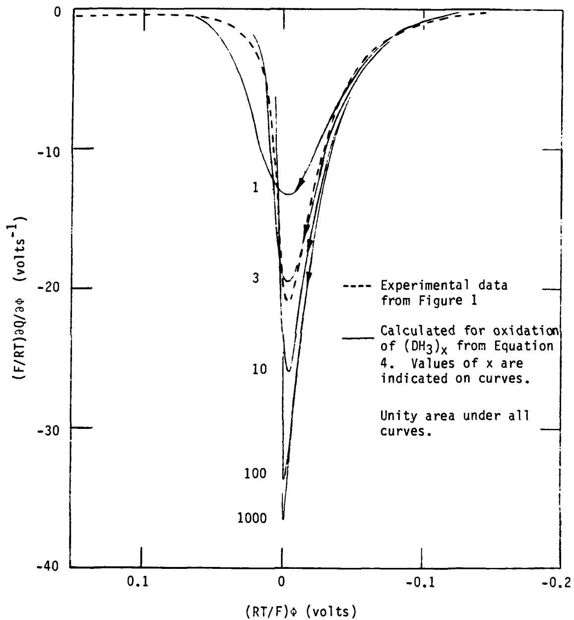
Figure 2. Experimental and Theoretical Voltammograms for Oxidation of Dark Blue to Light Blue Form of Lutetium Diphthalocyanine.
