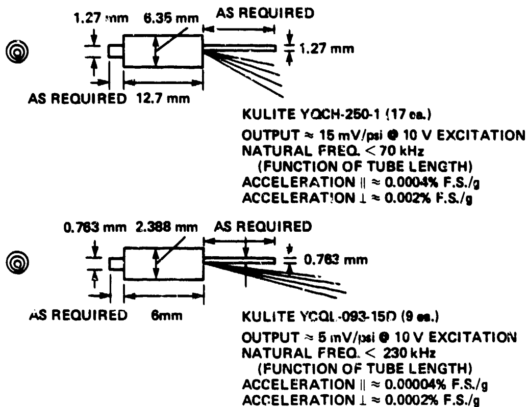
Figure 1 Pressure transducers for oscillating air foil
