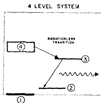
Figure 4. Schematic energy level diagram for the four-level system.
