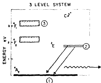
Figure 3. Energy level diagram for the three-level ruby system.
