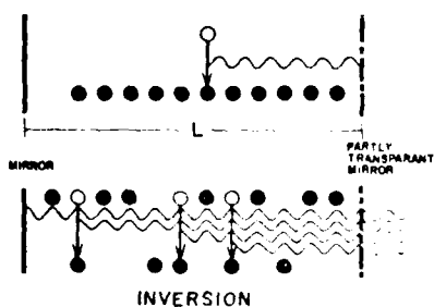
Figure 5. Shown in all is the optical cavity with the medium slightly excited. In b, there is a marked population inversion. Some levels are stimulated to emit.
