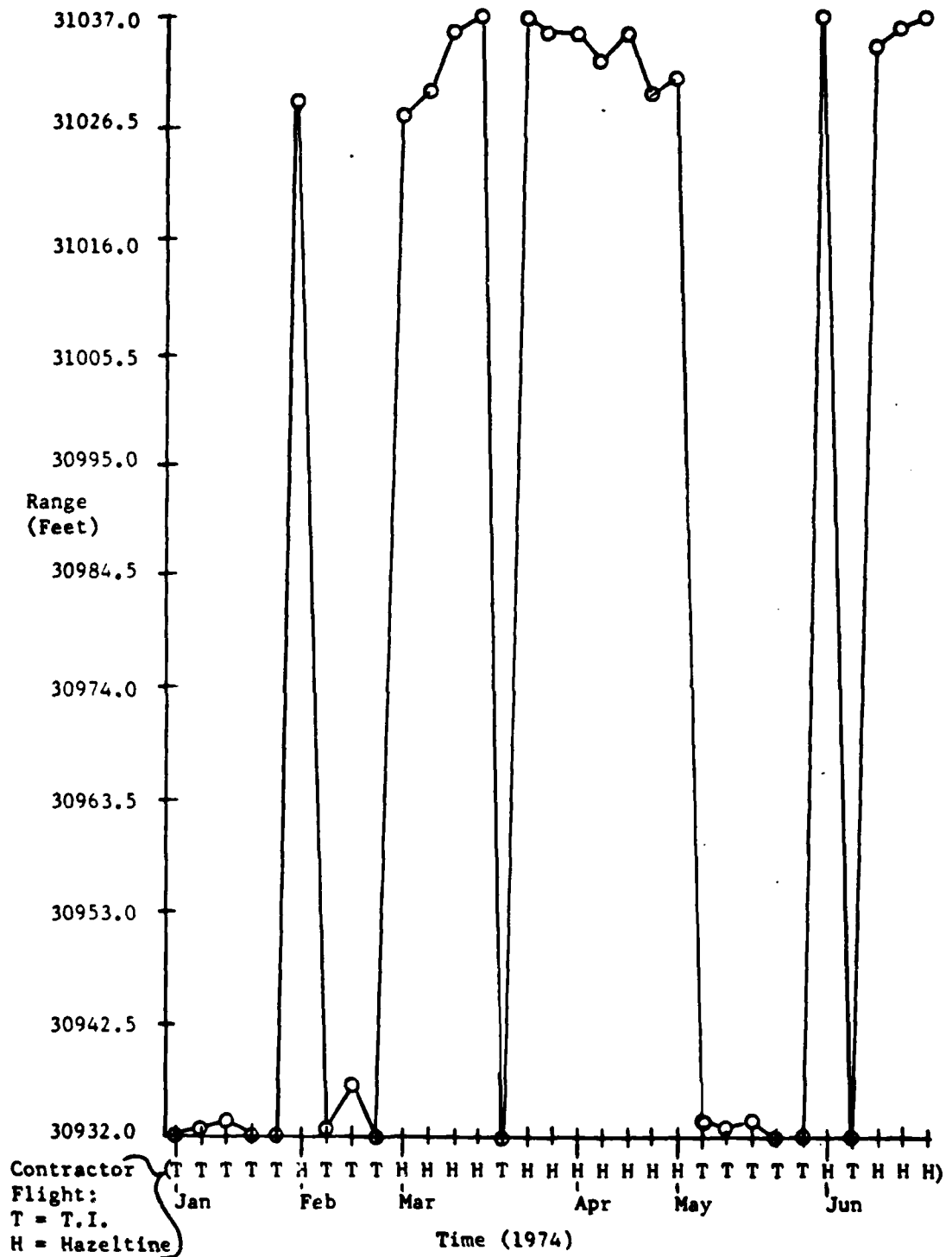
Figure III-6: Range Pre-calibration Values Versus Time.
