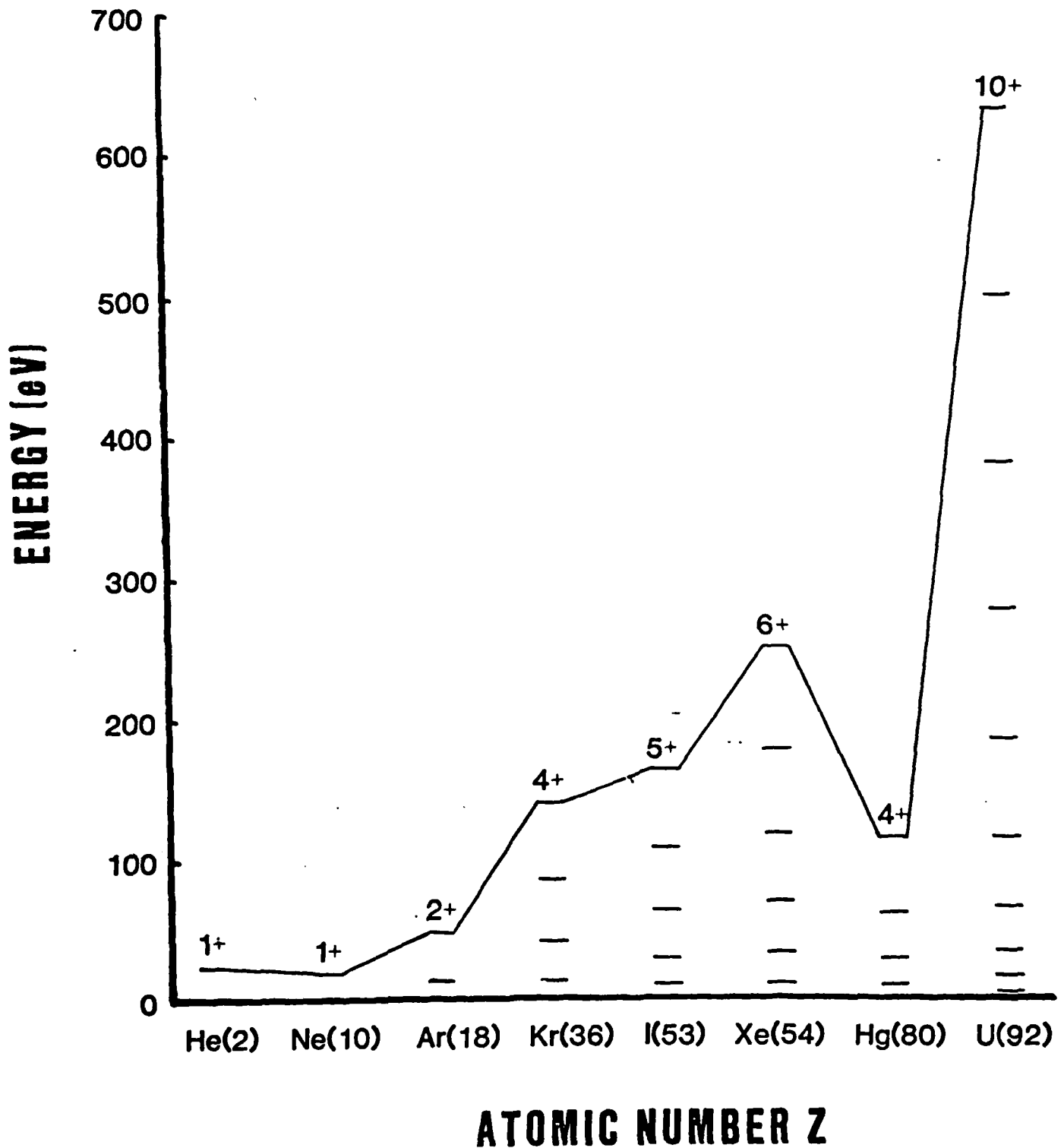
Fig. (9): Plot of the ionization energies representing the total energy transfer required for the production of different charge states as a function of atomic number (Z). The envelope curve is drawn to connect the states representing the maximum charge state observed.
