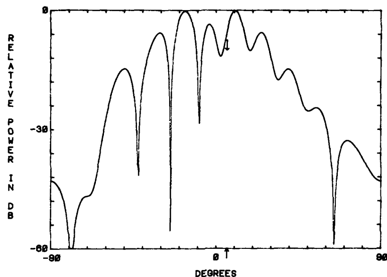
Figure 32a. Phase-Only Nulling in the Sum and Difference Channels Simultaneously in the Mainbeam of a Sum Pattern at 5°
