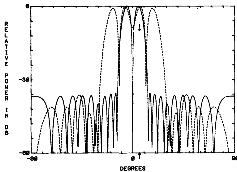
Figure 32d. Cancellation Beam From Phase-Only Nulling in the Sum and Difference Channels Simultaneously With a Jammer in the Mainbeam of the Difference Channel
