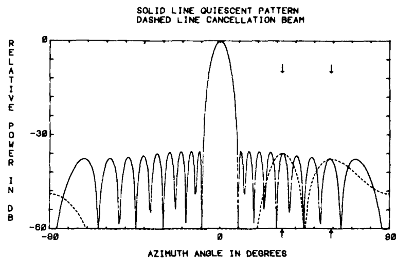
Figure 22c. Sum Channel Cancellation Beam From Amplitude and Phase Nulling in the Sum and Difference Channels Simultaneously
