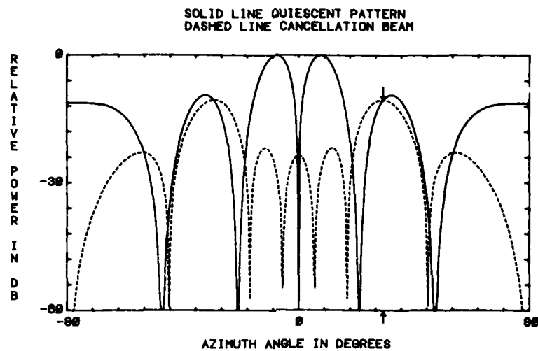
Figure 17c. Cancellation Beam From Phase-Only Nulling in the Difference Channel
