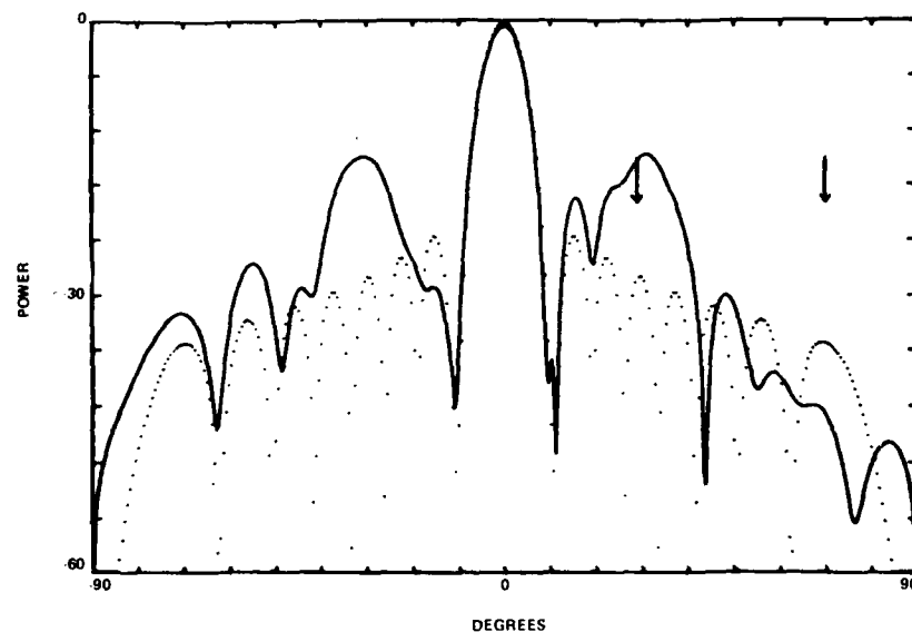
Figure 30c. Phase-Only Nulling in an 18-Element Low Sidelobe Array With 2 Percent Amplitude Error, 4^\circ Phase Error, 0.0001\lambda position Error, and 8-Bit Phase Shifters
