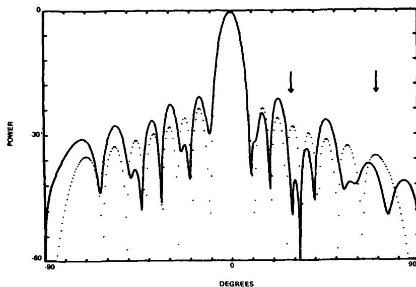
Figure 30b. Phase-Only Nulling in an 18-Element Low Sidelobe Array With 0.1 Percent Amplitude Error, 1^\circ Phase Error, 0.0001\lambda Position Error, and 8-Bit Phase Shifters
