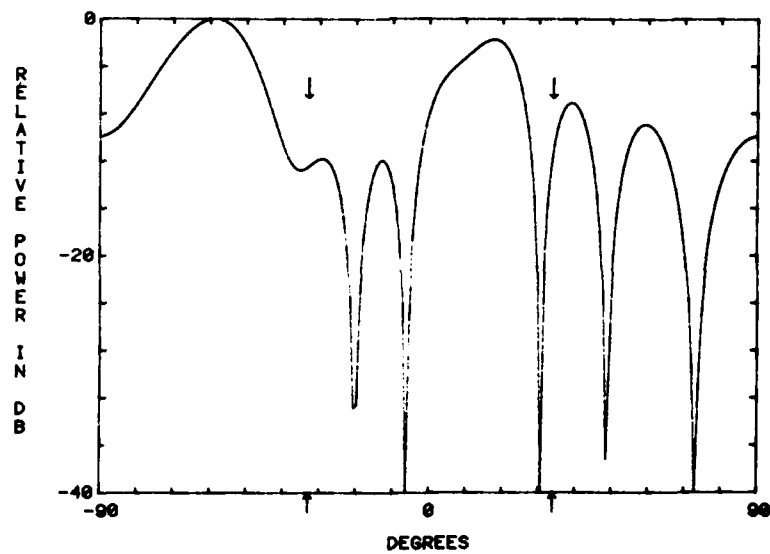
Figure 31b. Phase-Only Nulling With Nearly Symmetrical Jammers at -33 and -34^\circ
