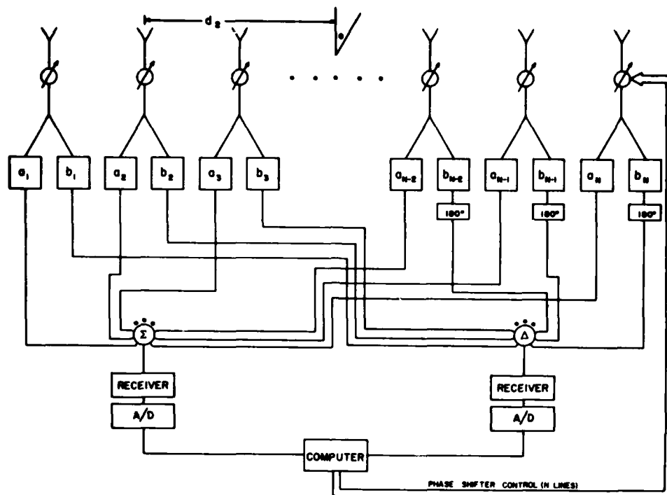
Figure 11. Monopulse Linear Array
