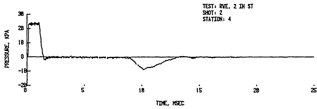
Figure 5. Pressure-time records - test section open, average input pressure 24.1 kPa
