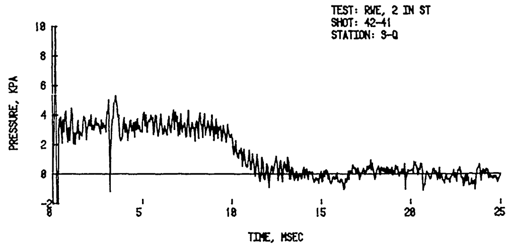
Figure A-4. (Continued) Pressure-time records for circular vented RWE - 10 holes
