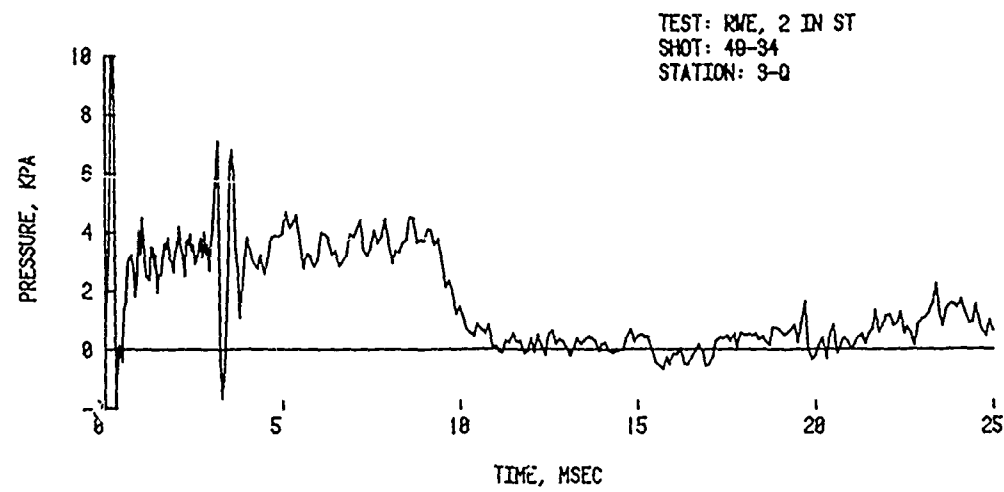
Figure A-3. (Continued) Pressure-time records for a single circular hole vented RVE
