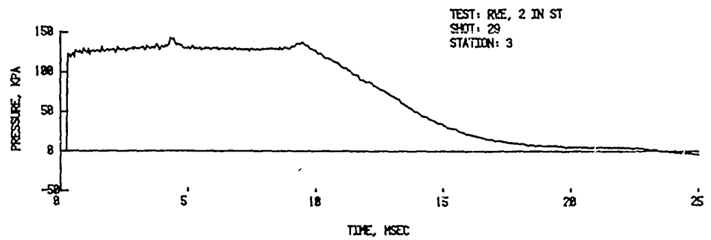
Figure A-2. (Continued) Pressure-time records for rectangular vented RVE.
