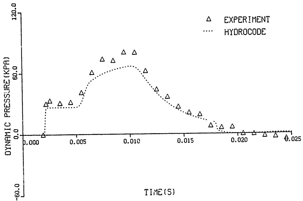
Figure 40. Comparison of experimental and computer side-on and dynamic records, 93.1 average kPa, no RWE, Station 3
