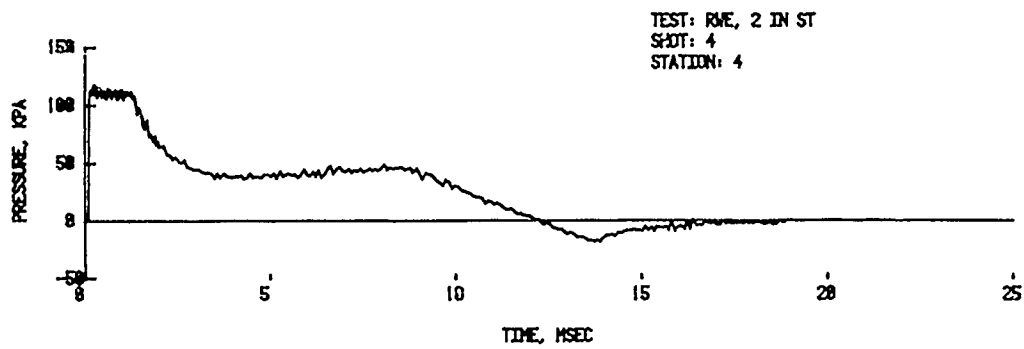
Figure 8. Pressure-time records - test section open, average input pressure 116.9 kPa
