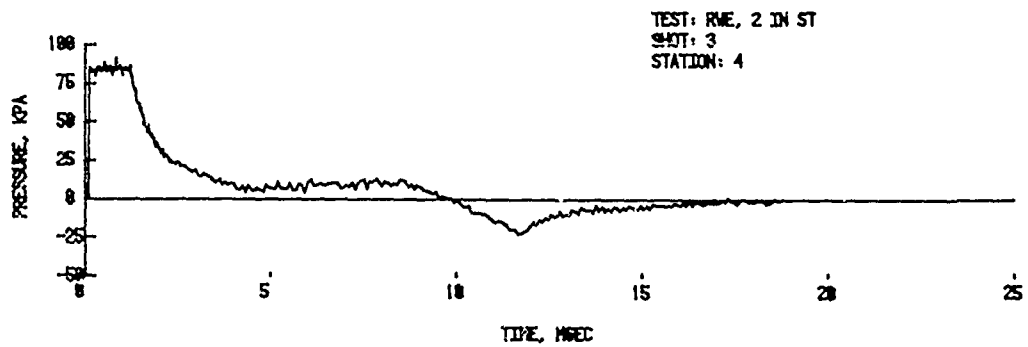
Figure 7. Pressure-time records - test section open, average input pressure 86.8 kPa
