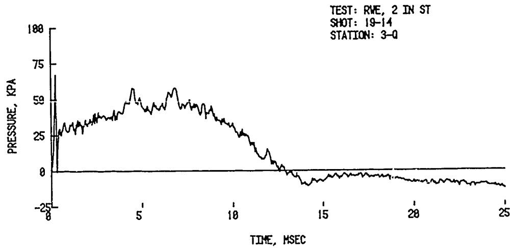
Figure 16. Stagnation pressure minus side-on - Type A solid plate RWE, average input pressure 91.9 kPa
