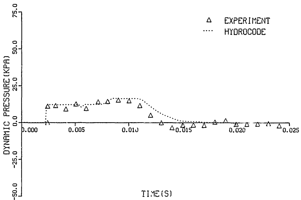
Figure 39. Comparison of experimental and computer side-on and dynamic records, 63.8 average kPa, RWE, Station 3
