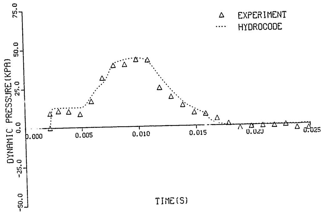
Figure 38. Comparison of experimental and computer side-on and dynamic records, 62.7 average kPa, no RWE, Station 3
