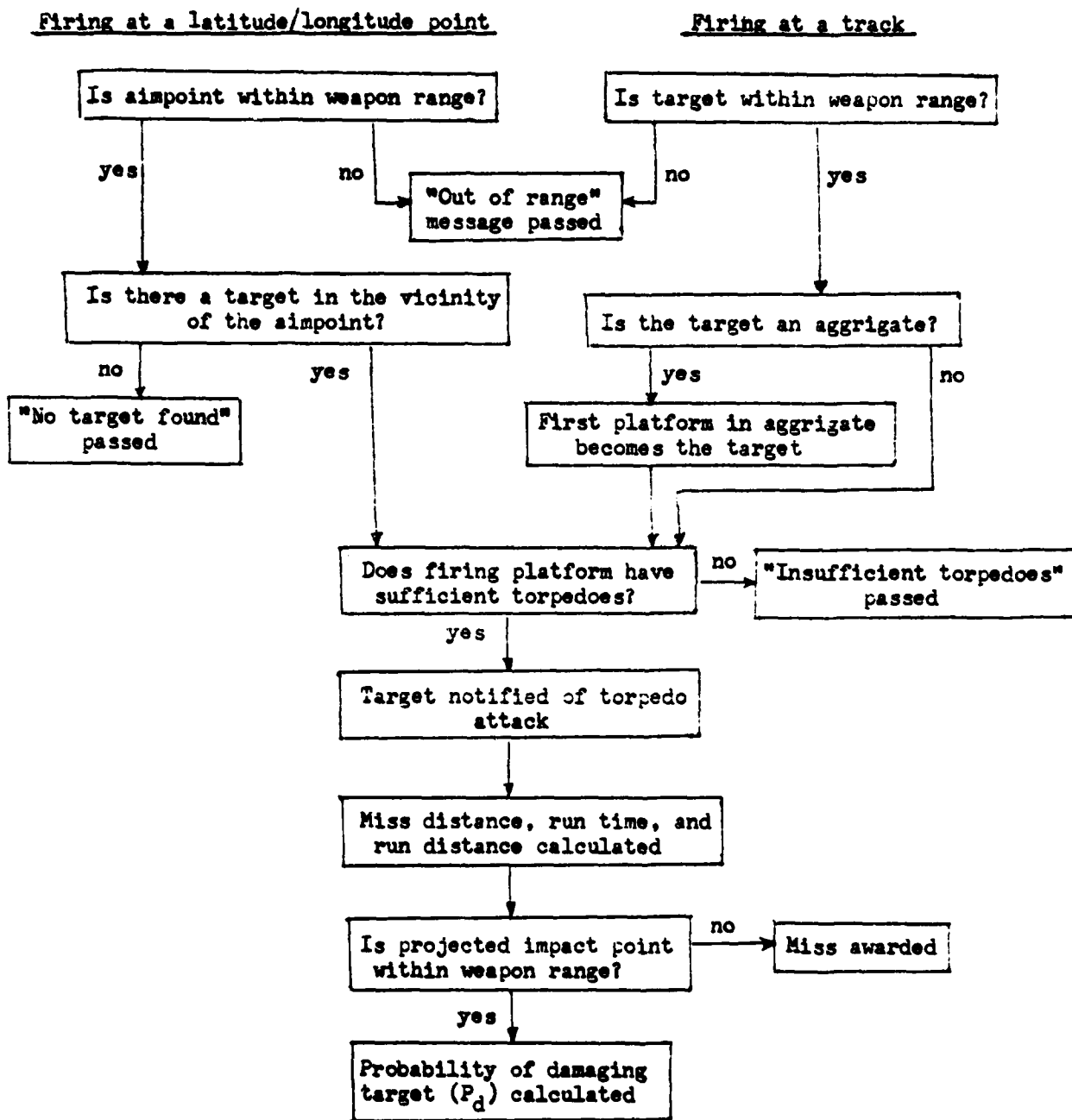
Figure 1. NWGS Torpedo Attack Model Flowchart.
