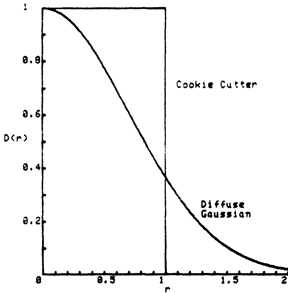
Figure 3. Damage Functions for Cookie Cutter and Diffuse Gaussian Weapons.
