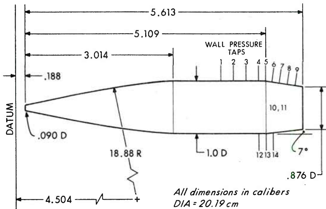
Figure 4. Boattailed Model Configuration
