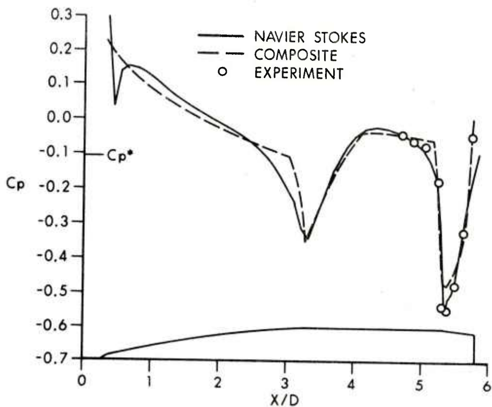
Figure 6. Comparison of Navier-Stokes, Composite and Experimental Surface Pressure Coefficients, M = 0.94
