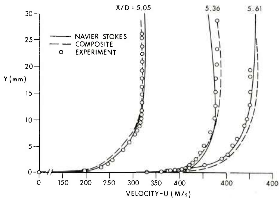
Figure 7. Velocity Profiles at X/D = 5.05 , 5.36 and 5.61 for M = 0.94 , \alpha = 0^\circ
