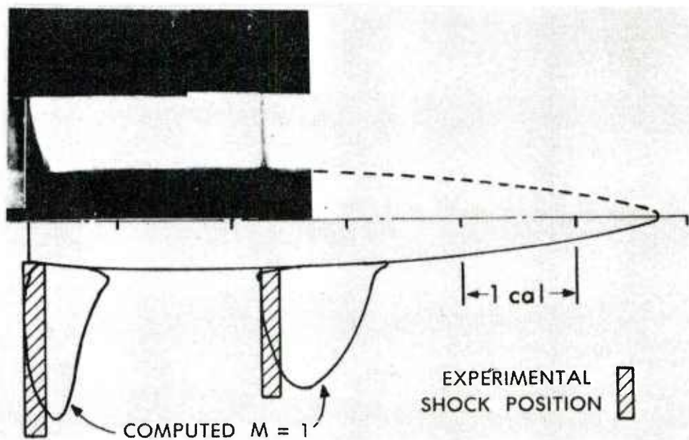
Figure 11. Boattail Shock Formation from Computer Mach Number Contours and Schlieren Photo
