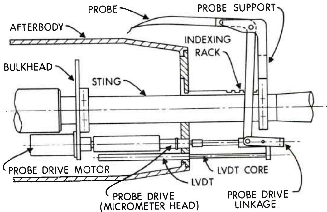
Figure 5. Afterbody of Wind Tunnel Model Showing Probe Support Mechanism
