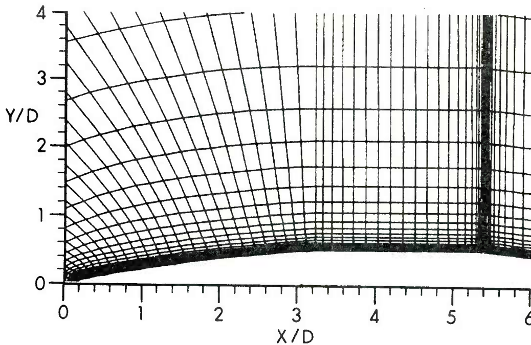
Figure 2b. Physical Grid for Navier-Stokes Computations - Expanded View Near Model
