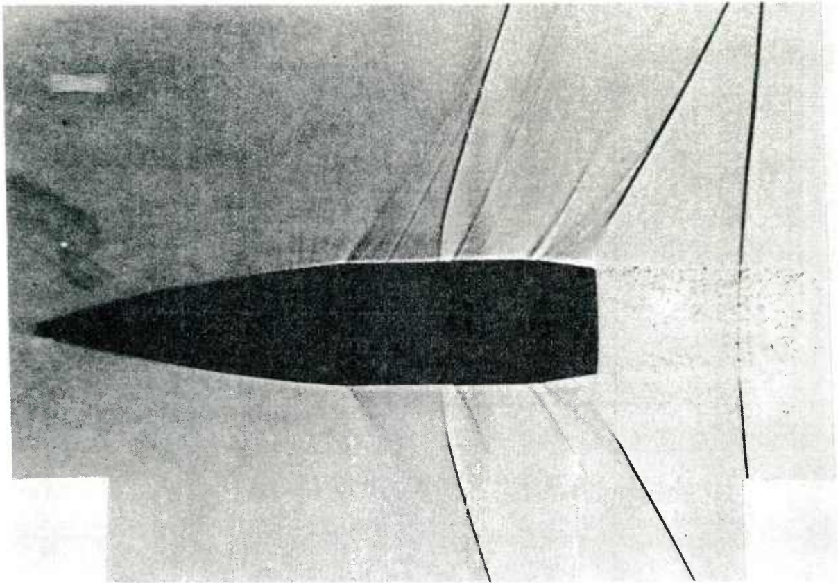
Figure 1. Spark Shadowgraph of Projectile at Transonic Velocity, M \approx .98
