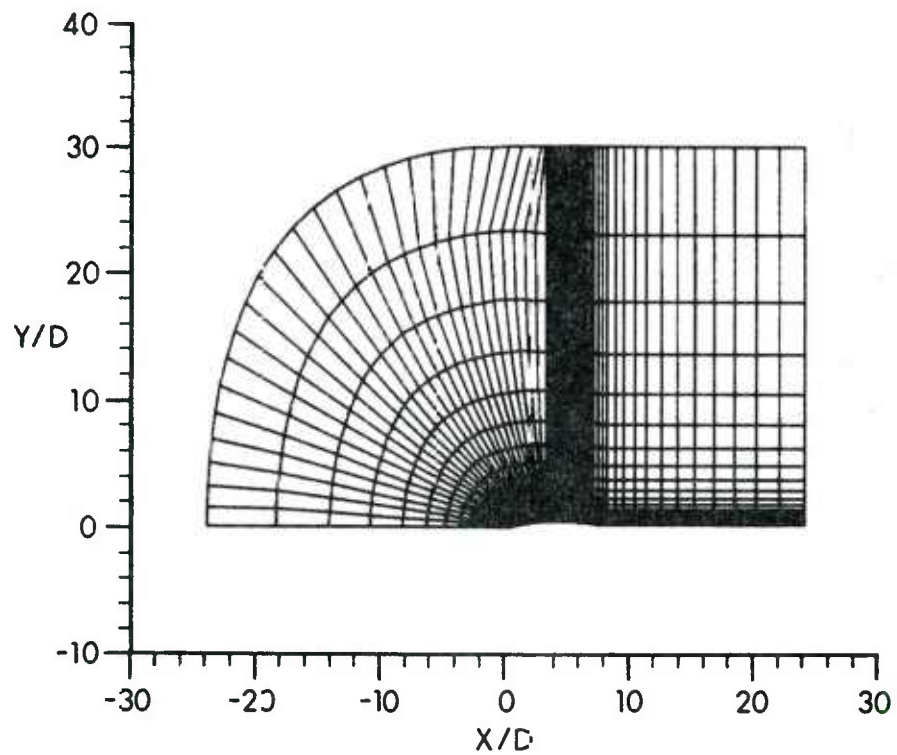
Figure 2a. Physical Grid for Navier-Stokes Computations - Full Grid
