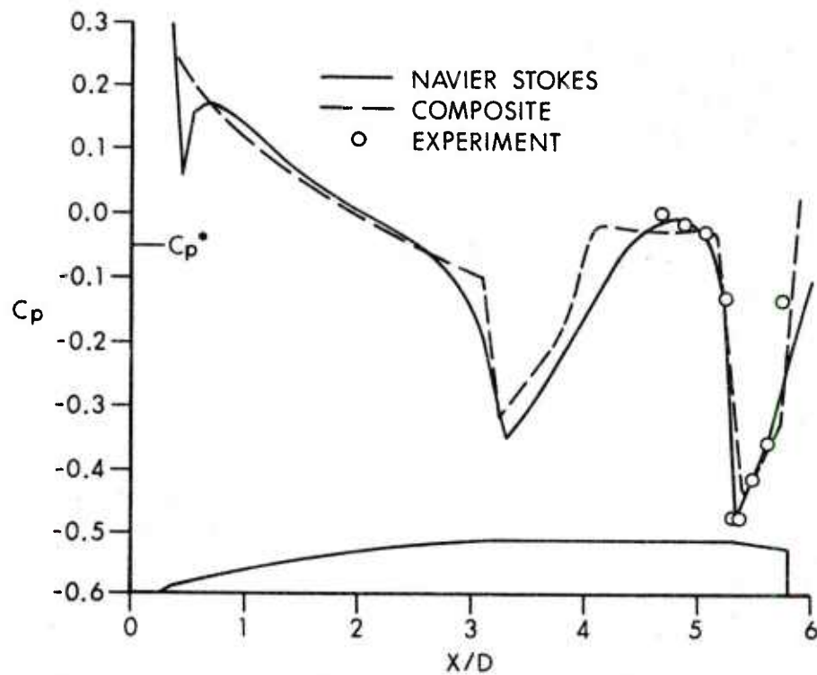
Figure 9. Comparison of Navier-Stokes, Composite and Experimental Surface Pressure Coefficients, M = 0.97 , \alpha = 0^\circ
