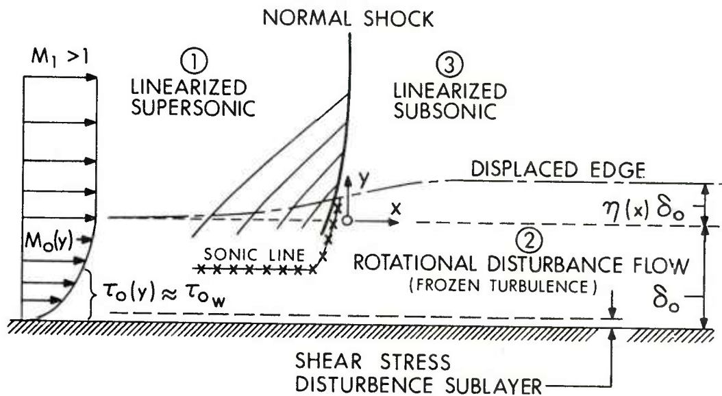
Figure 3. Triple Deck Model of Shock Boundary Layer Interaction
