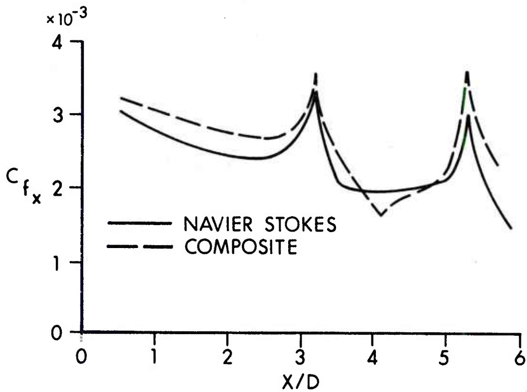
Figure 12. Comparison of Skin Friction Coefficient Between Navier-Stokes and Composite Solution Technique M = 0.97 , \alpha = 0^\circ
