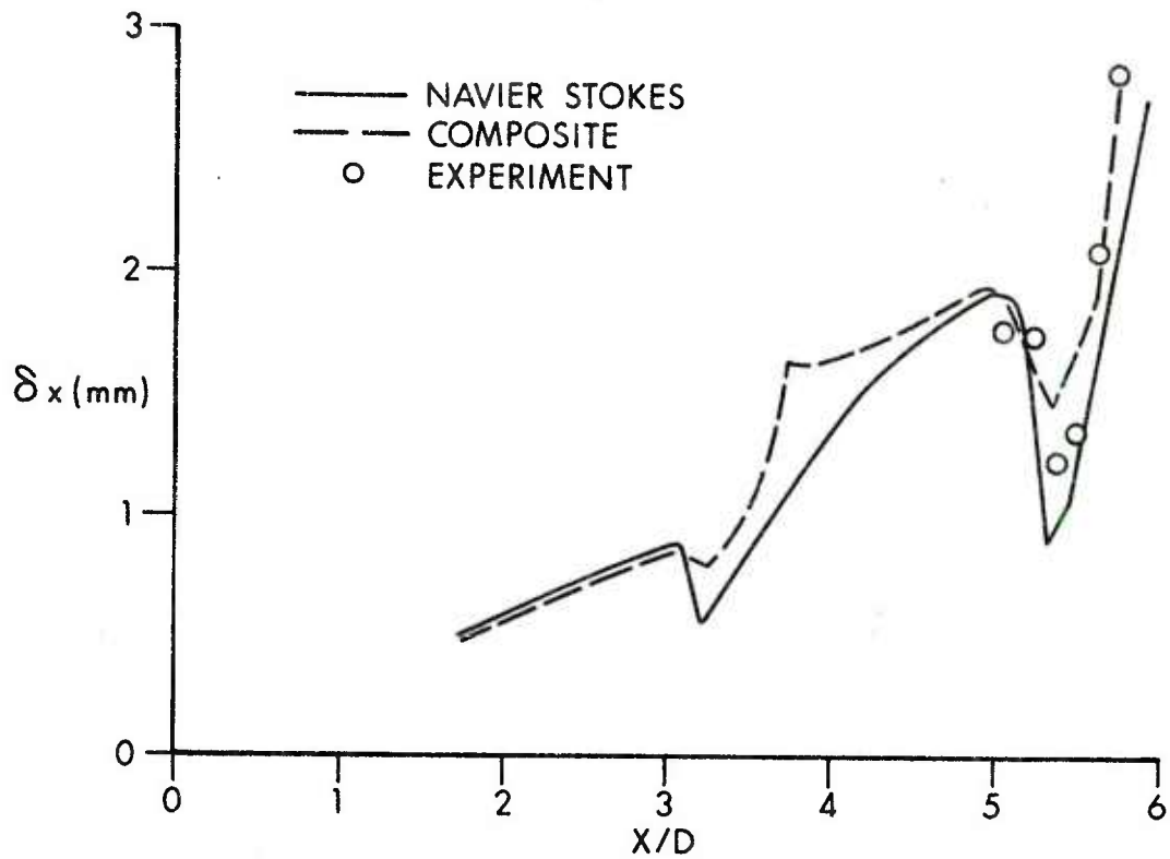
Figure 8. Comparison of Displacement Thicknesses: Experiment, Navier-Stokes and Composite, M = 0.94 , \alpha = 0^\circ
