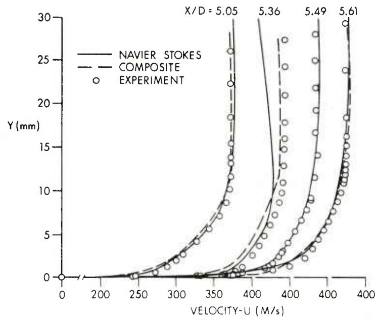
Figure 10. Velocity Profiles at X/D = 5.05, 5.36, 5.49 and 5.61 for M = 0.97, \alpha = 0^\circ
