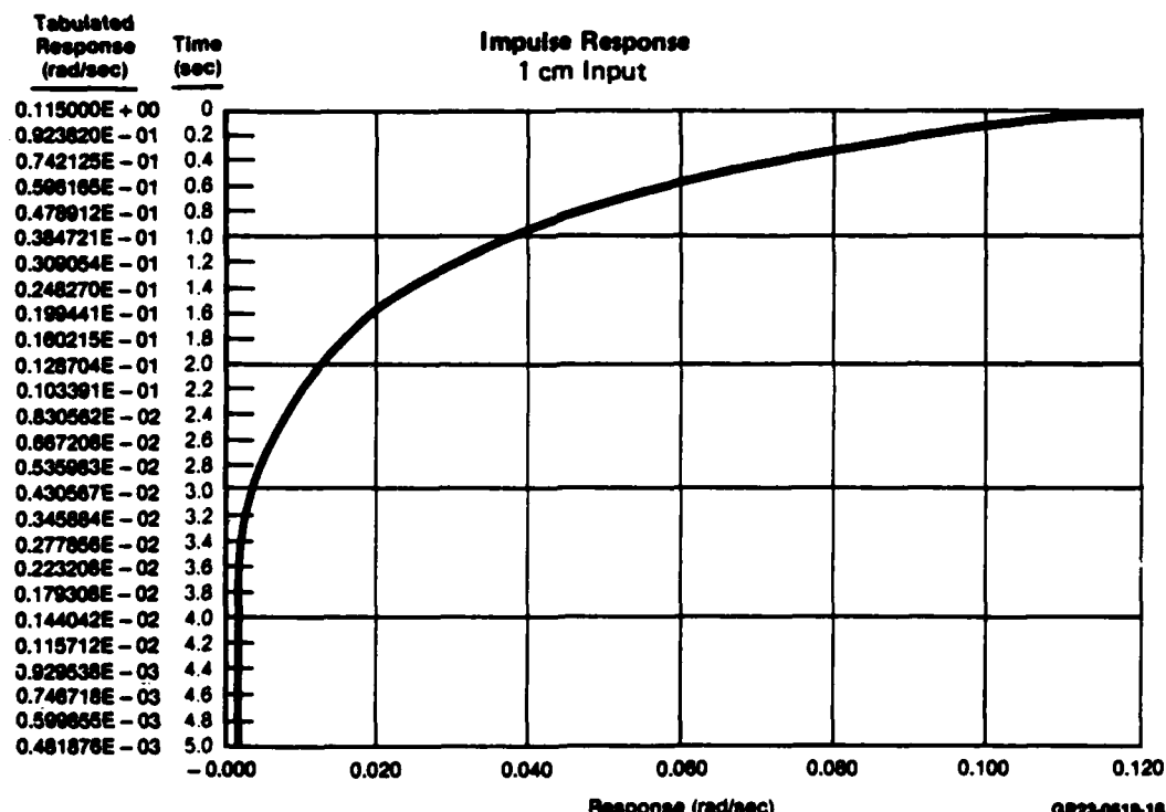
Figure 12. Directional Dynamics, \ddot{\psi}/\delta_{\text{PED}}
