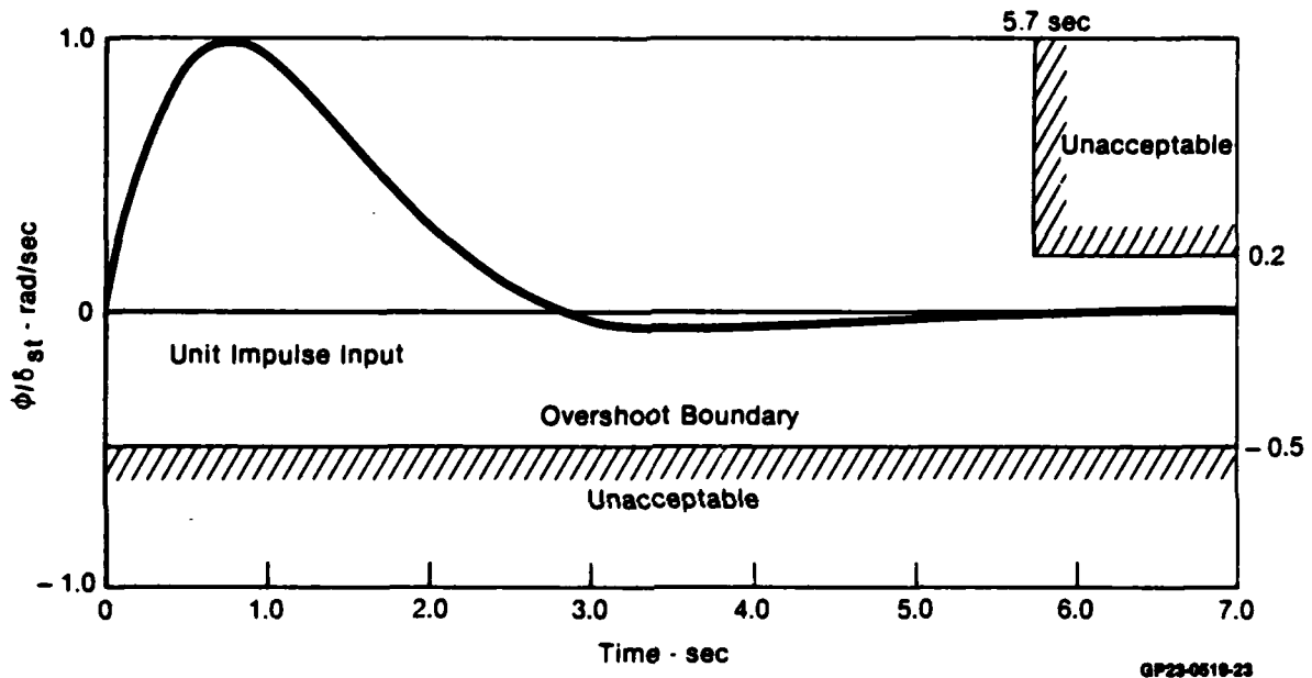
Figure A-2b. Frequency and Time Response Configuration TR1 \zeta = 0.667 \omega_n = 1.5 \text{ rad/sec}
