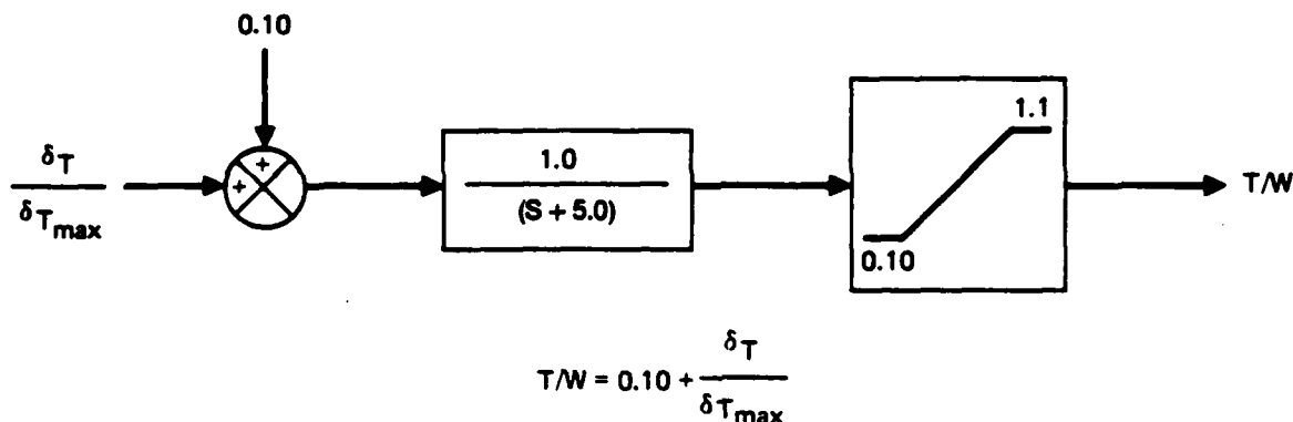
Figure 13. Thrust-to-Throttle Dynamics
