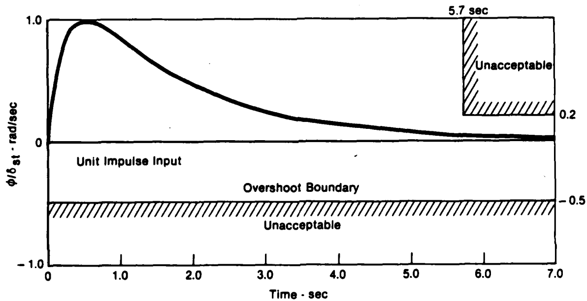
Figure A-7b. Frequency and Time Response Configuration TR6 \zeta = 1.57 \omega_n = 1.75 \text{ rad/sec}
