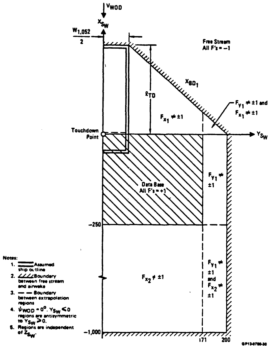
Figure D2. Definition of Data Base Extrapolation Boundaries in the X_{SW} - Y_{SW} Plane for \psi_{WOD} = 0 Deg
