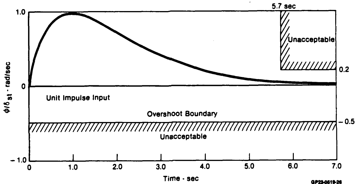
Figure A-5b. Frequency and Time Response Configuration TR4 \zeta = 1.0 \omega_n = 1.0 rad/sec
