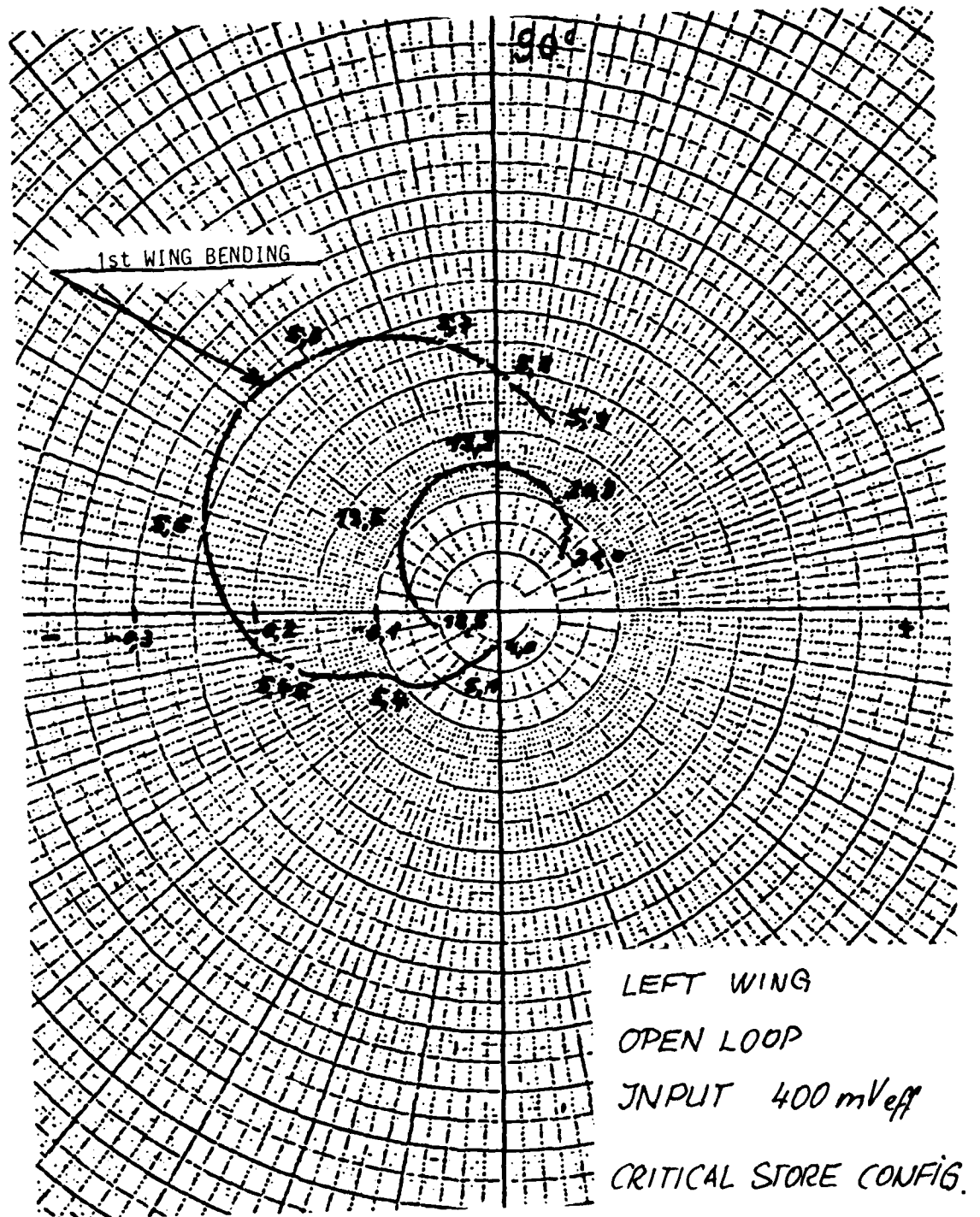
Figure 6. Structural Mode Coupling Test with Critical Store, Left Wing
