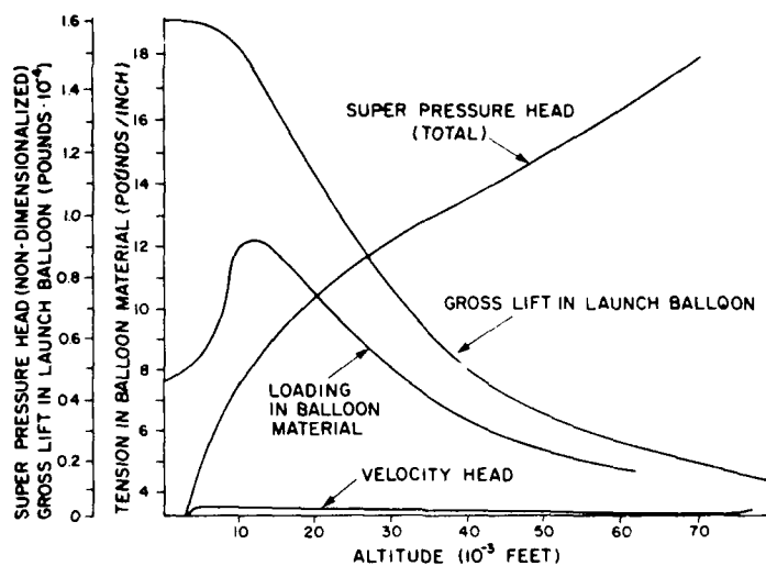
Figure C3. Stratoscope II Launch Balloon Gas Transfer
