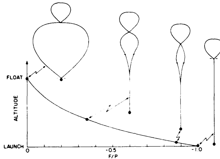
Figure C2. Variation of the Shape of a Tandem-Balloon System as it Ascends to Altitude. The short lines indicate the zero pressure level. F is the net upward force on the main balloon apex and P is the system payload
