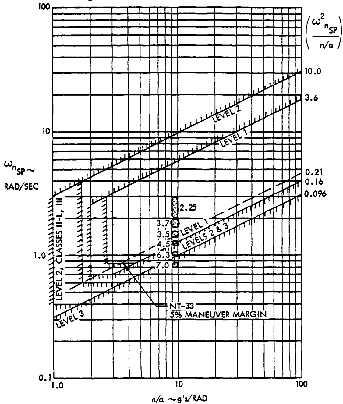
Figure 24 NT-33 Category C Data Compared to MIL Spec 5% Maneuver Margin
