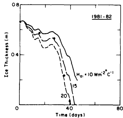
Figure 1 (cont'd). Predicted ice thicknesses during the decay period starting from maximum observed ice cover thickness and using different H_{01} values. The plotted points are observed thicknesses.
