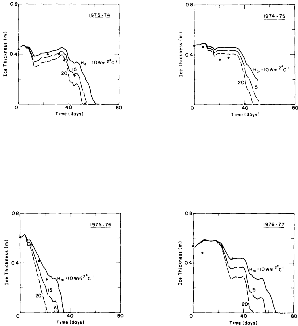
Figure 1. Predicted ice thicknesses during the decay period starting from maximum observed ice cover thickness and using different H_{0i} values. The plotted points are observed thicknesses.
