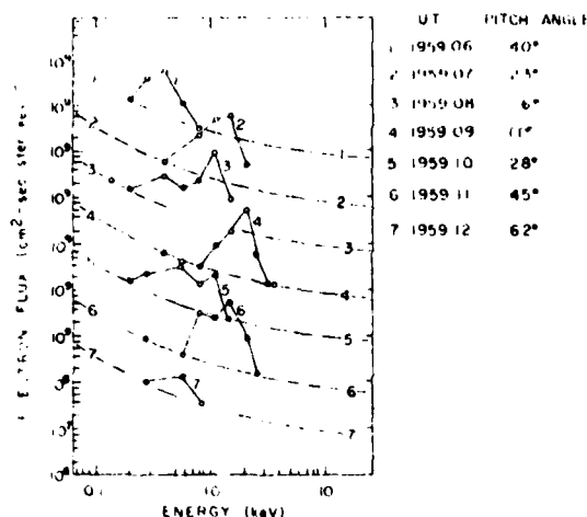
Fig. 5. Directional, differential flux measurements during event 4. The format is the same as Figure 4.
