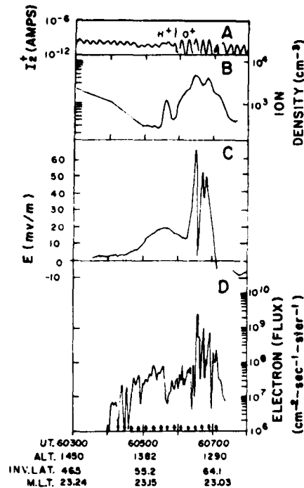
Fig. 2. Simultaneous measurements of (a) the current to ion sensor, (b) the ion density, (c) the 5-s-averaged values of the electric field, and (d) the directional electron flux ( 80 \text{ eV} \leq E \leq 17 \text{ keV} ). The arrows at the bottom of the plot indicate times when the energetic electron spectrometer was looking upward along magnetic field lines. Data are plotted as functions of universal time in seconds of the day.
