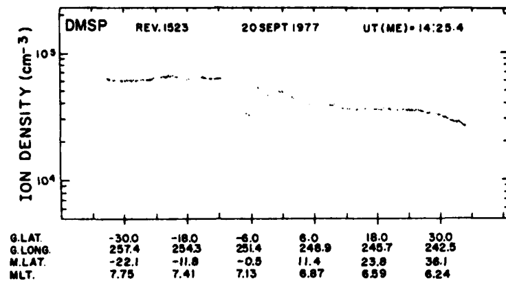
Fig. 2. An example of equatorial spread F observed near 0700 LT at 840 km. Ion density is plotted as a function of geographic latitude and longitude, magnetic latitude, and magnetic local time.
