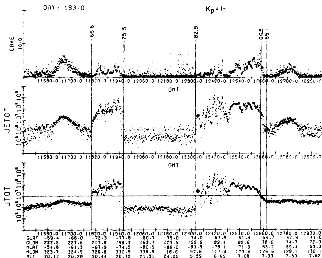
Fig. 1. Integral flux in (\text{cm}^2 \text{ sr s})^{-1} (bottom panel), energy flux in \text{keV} (\text{cm}^2 \text{ sr s})^{-1} (middle panel), and average energy in \text{keV} (top panel) of precipitating electrons measured by the DMSP/F2 satellite passing over the south pole on July 2, 1978. These values are plotted as functions of universal time (in seconds), geographic latitude and longitude of the subsatellite position, corrected geomagnetic latitude and longitude of the satellite position projected along a Jensen-Cain magnetic field to 100 km, and magnetic local time. The vertical lines indicate equatorward and poleward boundaries of precipitating auroral electrons.
