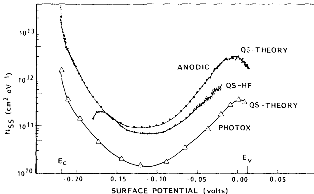
Figure 2. Surface State Density ( N_{SS} ) for PHOTOX ™ and Anodic Oxide Interface with \text{Hg}_{0.7}\text{Cd}_{0.3}\text{Te} . Anodic curves calculated by two different methods from the same data. PHOTOX ™ curve used method which gave higher anodic curve.
