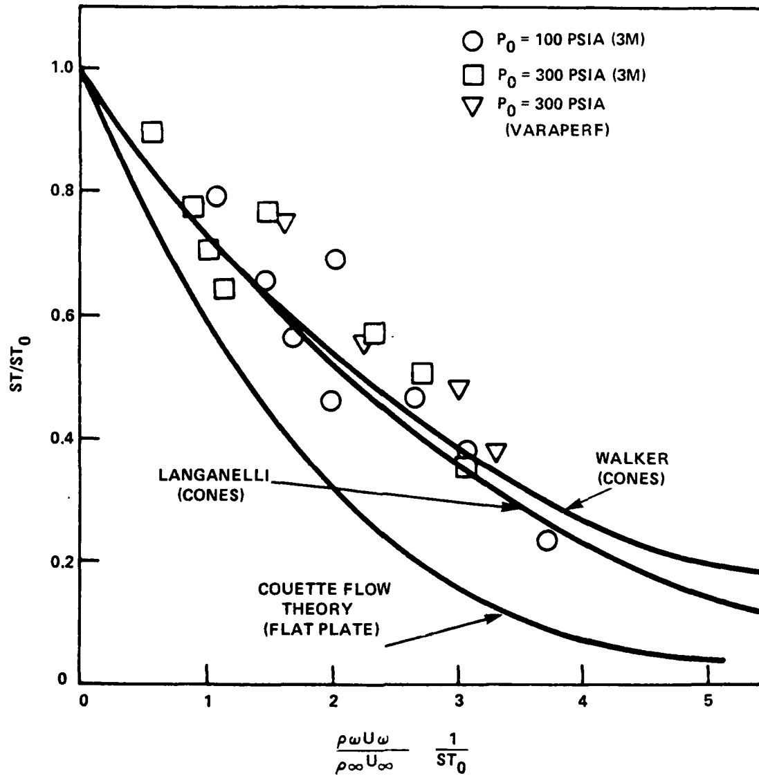
FIGURE 42. COMPARISON OF EXPERIMENT TO THEORY (SYMMETRIC BLOWING)
