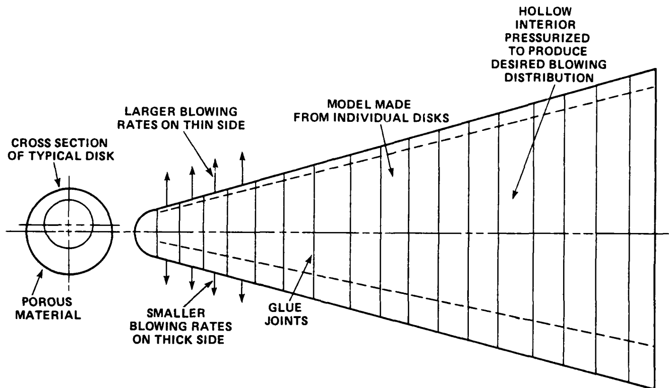
FIGURE 4. SCHEMATIC OF BLOWING MODEL DESIGN
