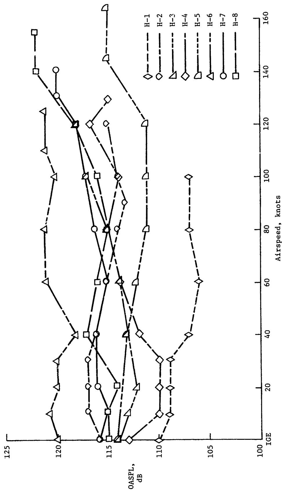
Figure 8.- Variation of overall sound pressure level (OASPL) with airspeed.
