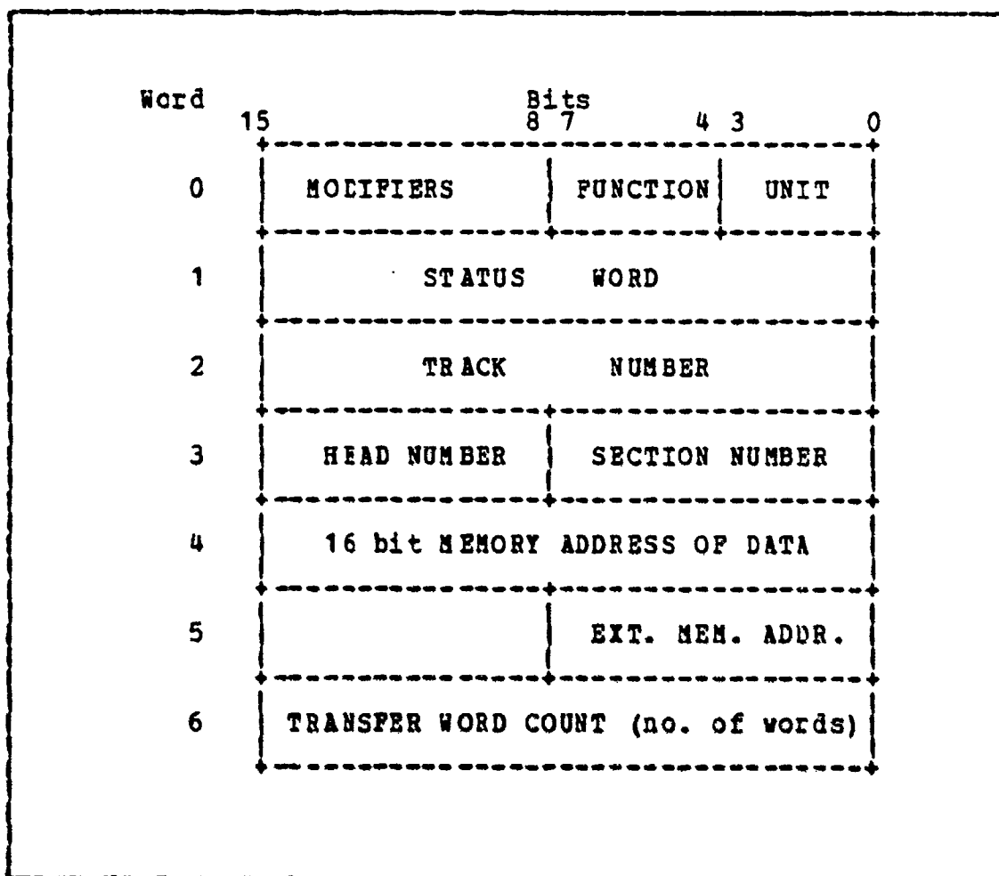
Figure 2.2 REMEX Read/Write Message Format.
