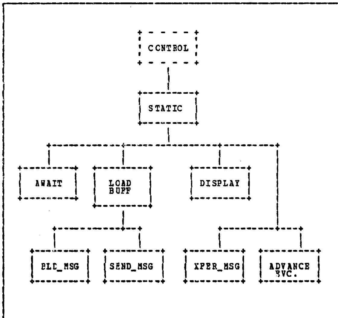
Figure 2.4 Static Model Design.
