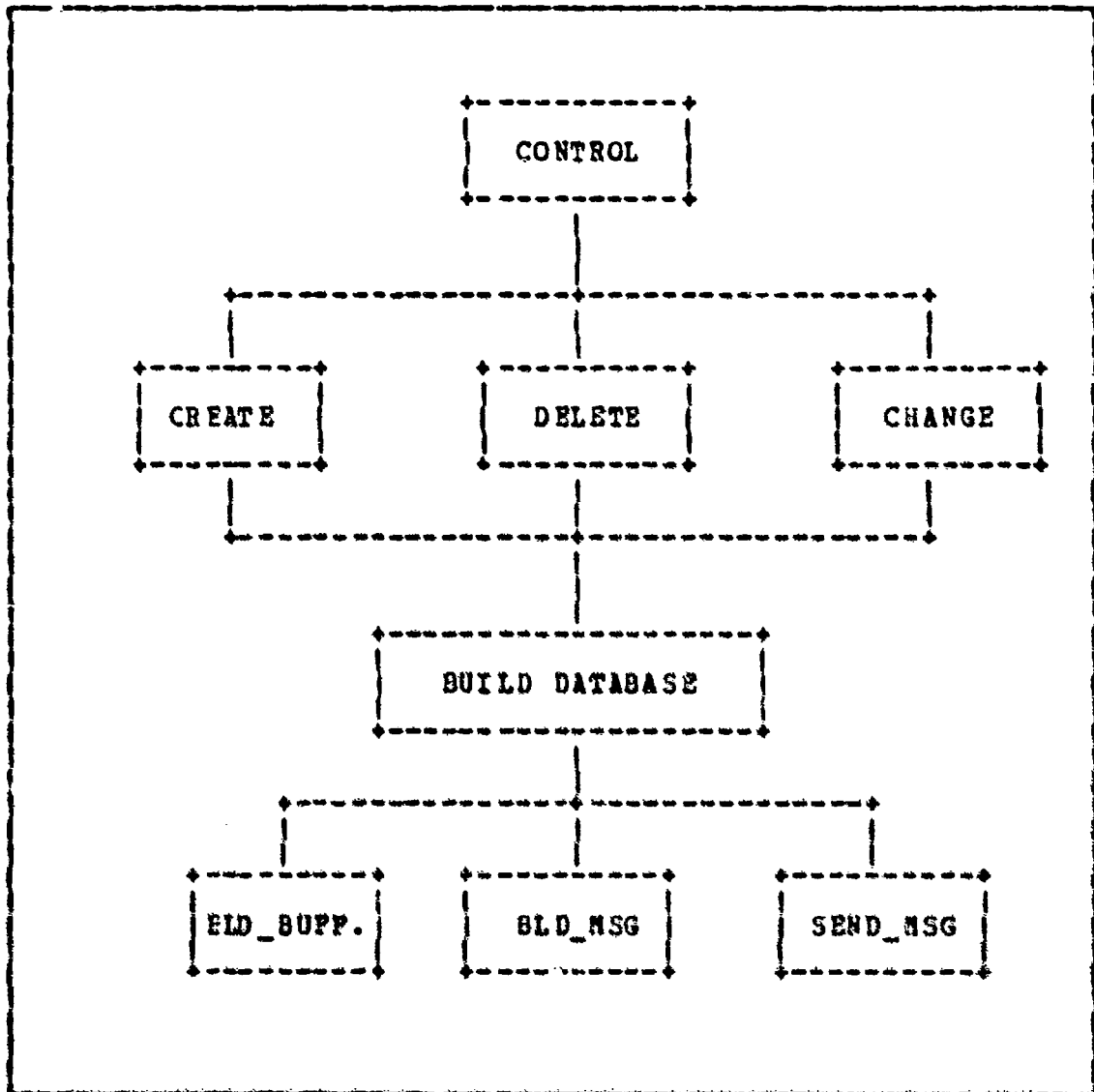
Figure 2.3 Database Design.
