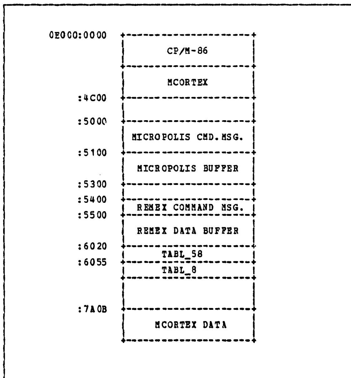
Figure 2.1 Common Memory Map.
