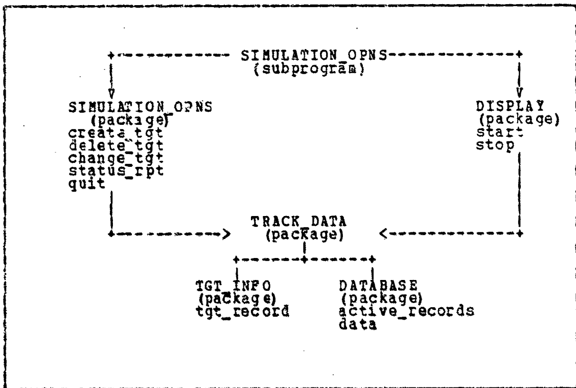
Figure B.1 Object-Oriented System Graph.
