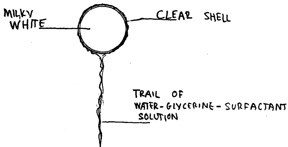
FIG. 11a EMULSION DROP DURING INITIAL STAGES OF ASCENT
