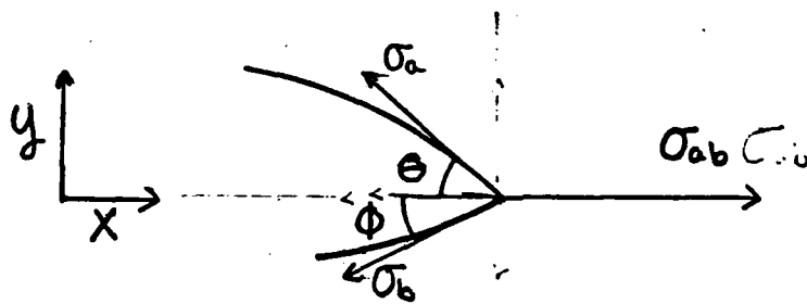
FIG. 6b. FORCE BALANCE AT BUBBLE EDGE
