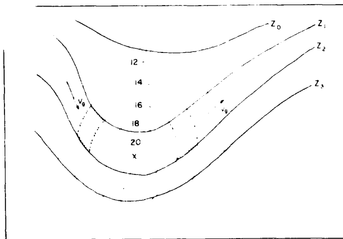
Fig. 3.1. Schematic showing vorticity advection by the geostrophic wind ( V_g ). Solid lines are height contours ( z ), dashed lines are contours of absolute vorticity (in units of 10^{-5} \text{ s}^{-1} ). Where the height and vorticity contours intersect, they form quadrilaterals (with curved sides). The strength of the advection is proportional to the number of such quadrilaterals per unit area. Where vorticity and height contours are parallel, no advection is occurring. The hatched quadrilateral is in a region of negative vorticity advection (NVA) by V_g , since V_g is pointing from lower to higher vorticity. The stippled quadrilateral is in a region of positive vorticity advection (PVA) by V_g .
