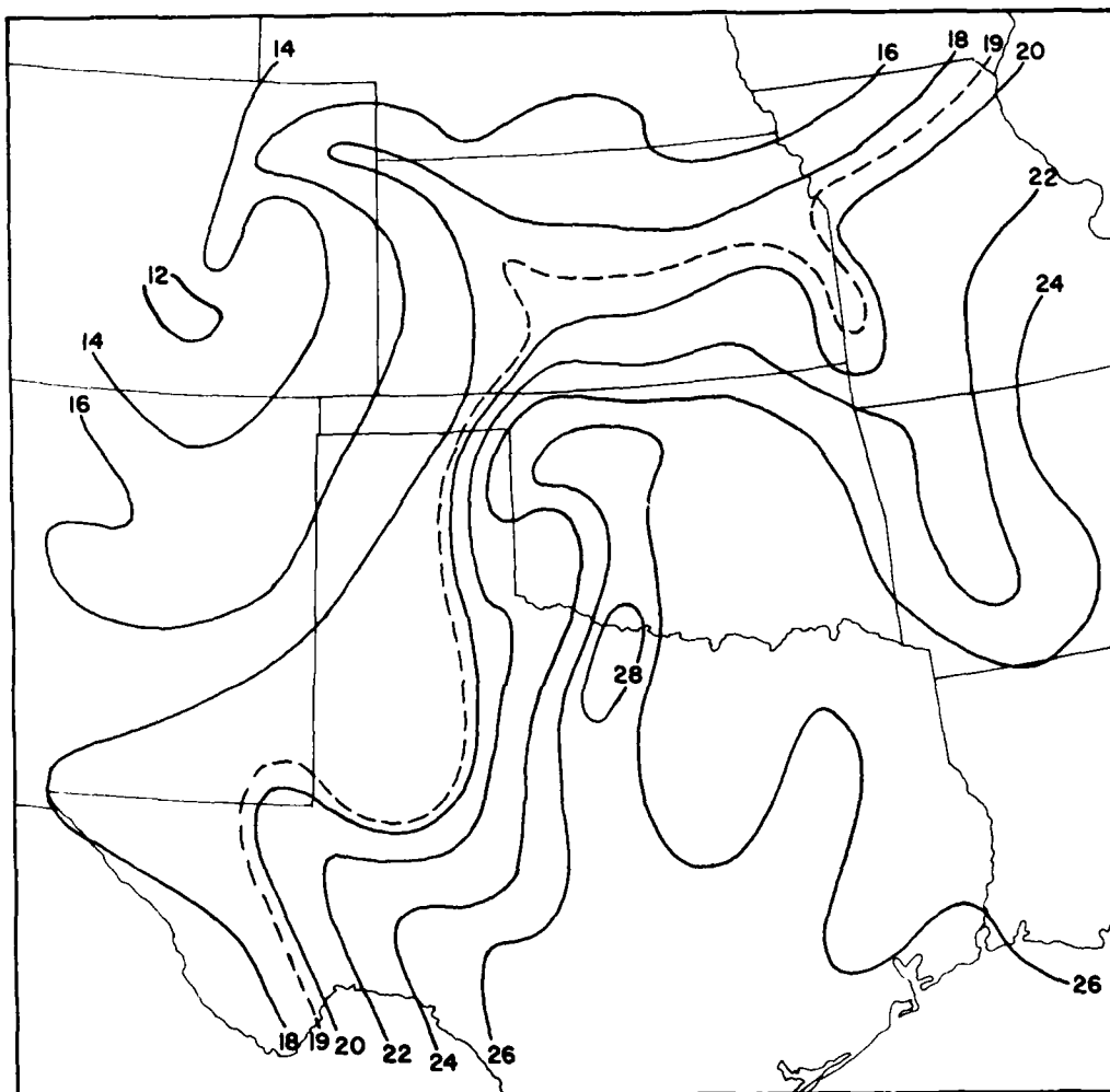
Fig. 3.4. Isotherms of \theta_p ( ^{\circ}\text{C} ) for data in Fig. 3.1.
