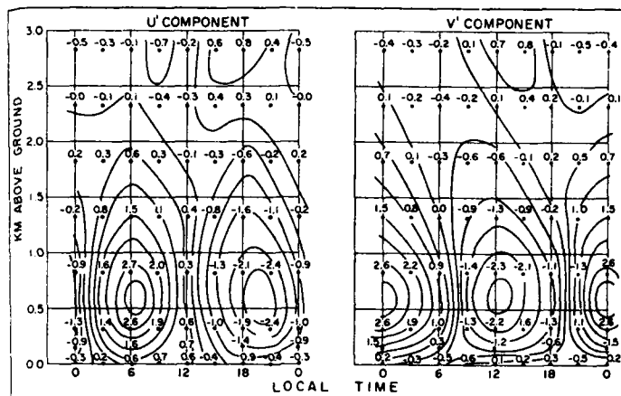
Fig. 3.33. Diurnal variation of wind components from their daily mean value at Fort Worth, Texas; values in \text{m s}^{-1} (after Bonner and Paegle, 1970).
