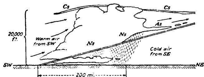
Fig. 3.8. As in Fig. 3.5, except for a warm front (after Byers, 1959).
