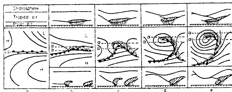
Fig. 1.2. Life cycle of extratropical cyclone (after J. Bjerknes, from Holte et al., 1957). In middle figures, thin lines are sea-level isobars. Top and bottom figures show schematic clouds, frontal surfaces and tropopause along lines \alpha , a little north and south of ETC center. The times from stages a to c and from c to e are roughly one day in each case.
