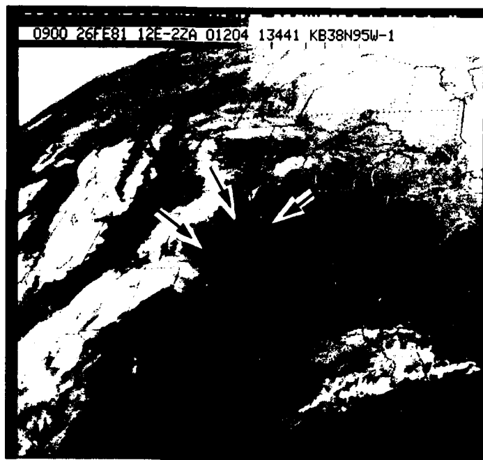
Fig. 3.36. Unenhanced infrared satellite image, showing the intrusion of moisture into eastern Kansas and western Missouri by means of "dark stratus" (arrows).
