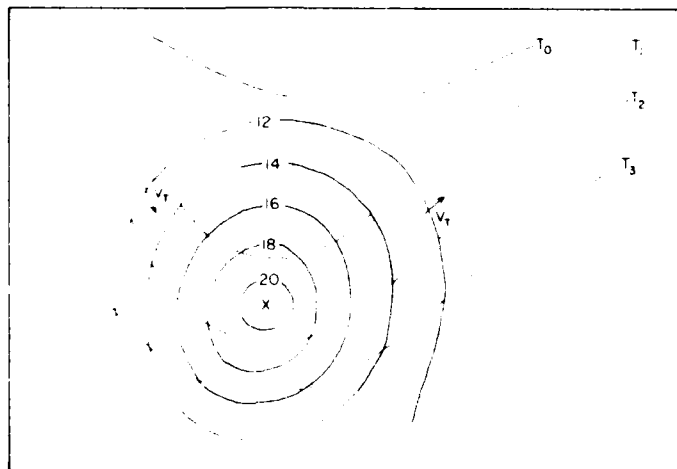
Fig. 2.1. Vorticity advection by the thermal wind ( V_T ). Thickness contours ( T ) are dashed lines, while solid lines are contours of absolute vorticity (as in Fig. 2.2). Note that thickness contours and height contours are not coincident, so that V_T differs from V_H .
