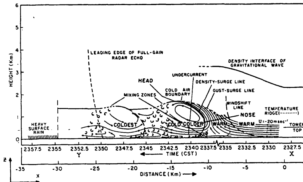
Fig. 3.18. Schematic cross section through thunderstorm outflow, showing relative depths and vertical structure of features (after Charba, 1974).
