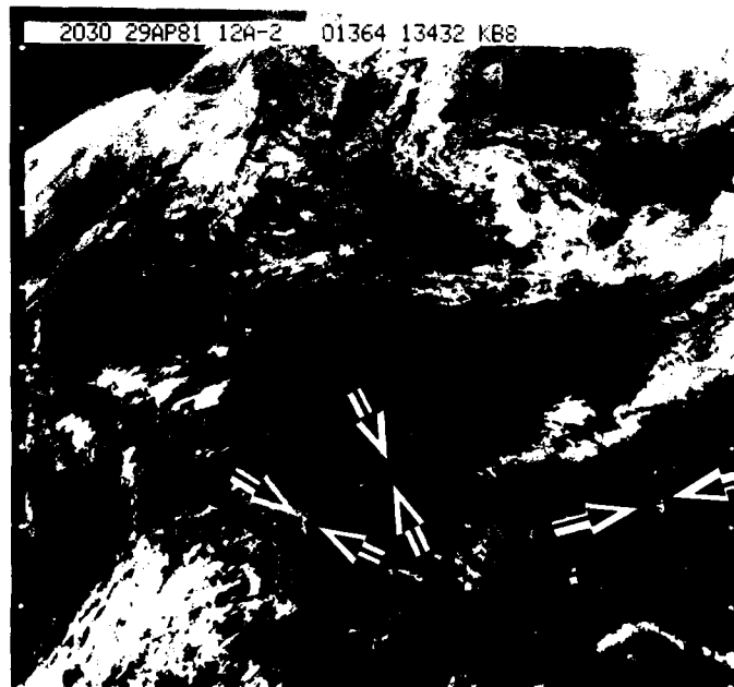
Fig. 3.16. Visible satellite image showing sea breeze-induced cloud lines along the Texas and Louisiana gulf coasts, and around the Florida peninsula as well (arrows).
