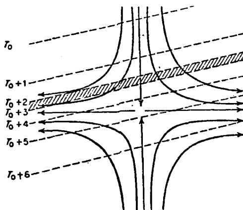
Fig. 4.6. Illustrating frontogenesis. The line of frontogenesis (hatched) moves toward the axis of dilatation, while the temperature contrast increases (after Petterssen, 1956a).
