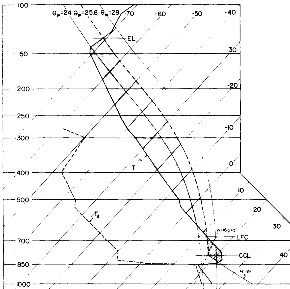
Fig. 1.11. Sample plotted sounding (Oklahoma City, Oklahoma, 1800 GMT, 12 Apr 1974) on a skew T-log p thermodynamic diagram. Heavy solid line is the temperature (T) observation during balloon ascent, heavy dashed line is for dewpoint ( T_d ). The thin solid line labelled \theta = 39 ( ^{\circ}\text{C} ) is the dry adiabath through the forecast maximum surface temperature, while the thin dashed line labelled w = 16 \text{ g kg}^{-1} is the mean mixing ratio in the lowest 100 mb. These intersect at the Convective Condensation Level (CCL). From the CCL, the parcel ascends along the pseudo-adiabath labelled \theta_w = 25.8 ( ^{\circ}\text{C} ), denoted by a dash-dot line. Pseudo-adiabaths labelled \theta_w = 24 and \theta_w = 28 are the thin solid lines included for reference. The ascending parcel is initially negatively buoyant and the negative area is depleted by hatching. As the parcel rises through the Level of Free Convection (LFC) it becomes positively buoyant, with the positive area stippled. After the parcel rises through the tropopause (about 150 mb) it once again crosses the environmental ascent curve, at the Equilibrium Level (EL).
