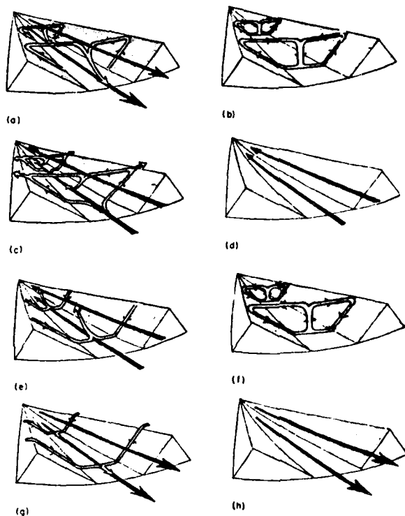
Fig. 3.31. Schematic illustration of the normal diurnal variations of the air currents in a valley, beginning at sunrise (a), and at about 3 h intervals through early morning (b-h) [after Defant, 1951].
