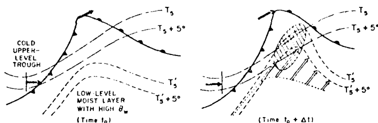
Fig. 2.5. Schematic illustration of differential advection (after Newton, 1980). Frontal symbols are conventional. Long-dashed lines are 500 mb isotherms while short-dashed lines are isotherms of low-level parcels lifted to 500 mb (proportional to \theta_w ). Note that the eastward progression of the 500 mb thermal trough and the northward progression of high \theta_w air in low levels creates a condition of instability at time t_0 + \Delta t in the hatched region. That is, low-level parcels in the hatched region, when lifted to 500 mb, are warmer than their environment.
