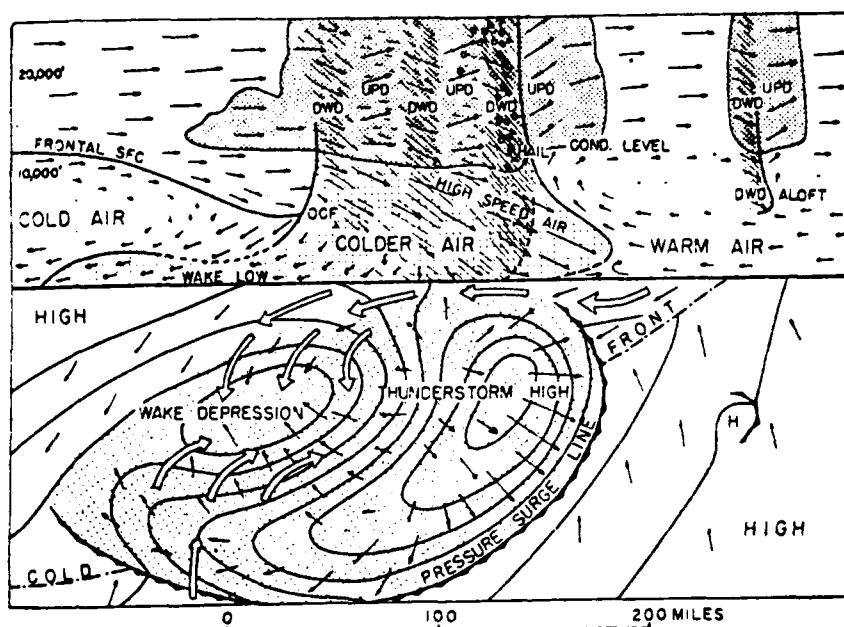
Fig. 8.11. Model of thunderstorm-induced mesoscale weather system (after Fujita, 1968). UPD denotes updraft, while DWD stands for downdraft.
