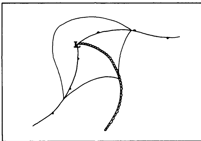
Fig. 3.14. Schematic example of triple point intersection of fronts and dryline in a developing frontal wave.
