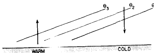
Fig. 4.7. Illustration of the effect of a direct circulation (warm air rising; cold air sinking) on horizontal gradients of potential temperature. The same picture arises if the air is rising (or sinking) everywhere, but the warm air is rising relative to the cold .
