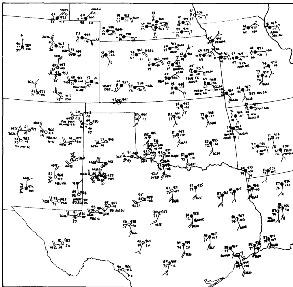
Fig. 3.1. Sectional plot of surface observations at 1800 GMT, 8 June 1974. Station model for plotted data given in Fig. 3.2.
