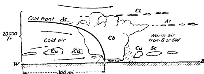
Fig. 3.5. Schematic cross section through cold front, showing cloud and precipitation (after Byers, 1959).
