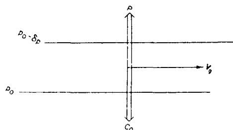
Fig. 1.3. The balance of forces for geostrophic equilibrium (after Holton, 1979). The pressure gradient force is denoted by P and the Coriolis force by C_0 , while the resultant geostrophic wind is V_g .
