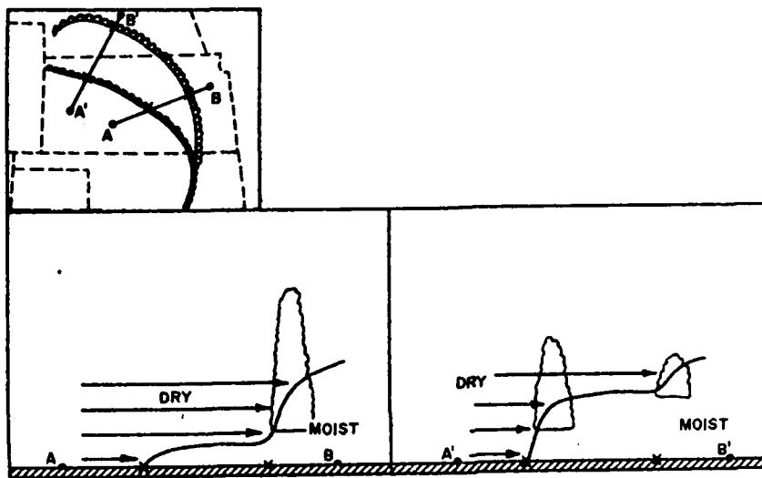
Fig. 3.13. Schematic cross sections along lines AB and A'B' showing different depths of moist layers in different locations along the dryline (after Siebers et al. , 1975). Clouds are indicative of convective intensity.
