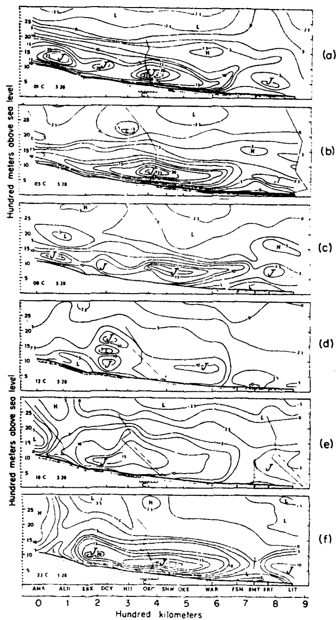
Fig. 3.35. Isotachs of southerly wind component ( \text{m s}^{-1} ) along the line from Amarillo, Texas (AMA) to Little Rock, Arkansas (LIT) during the day of 28 May 1961 (after Hoecker, 1963). Jet cores are indicated by "J" with other maxima and minima by an "H" or an "L", respectively.
