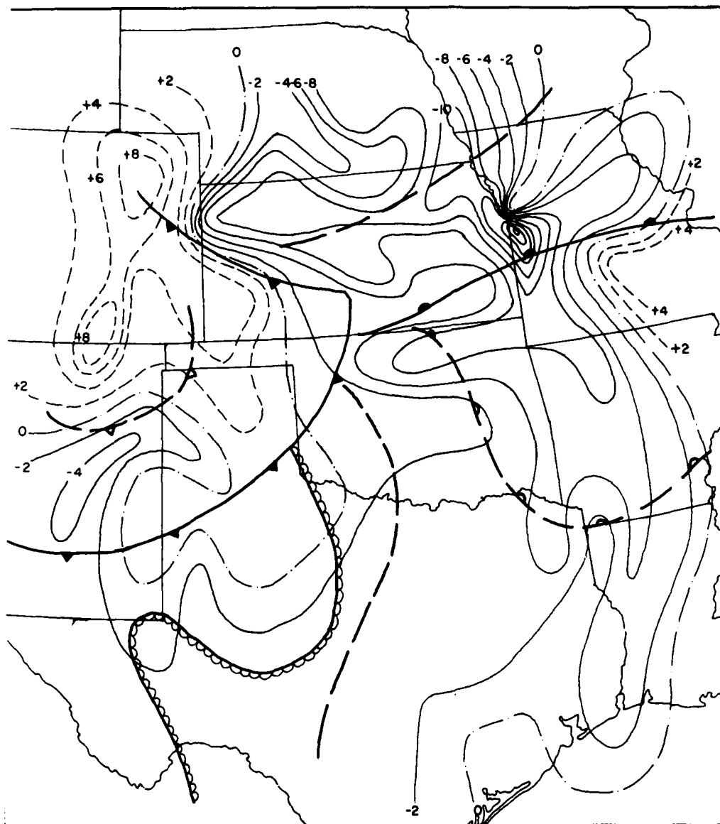
Fig. 3.29. As in Fig. 3.28 except at 2100 GMT, 8 June 1974.
