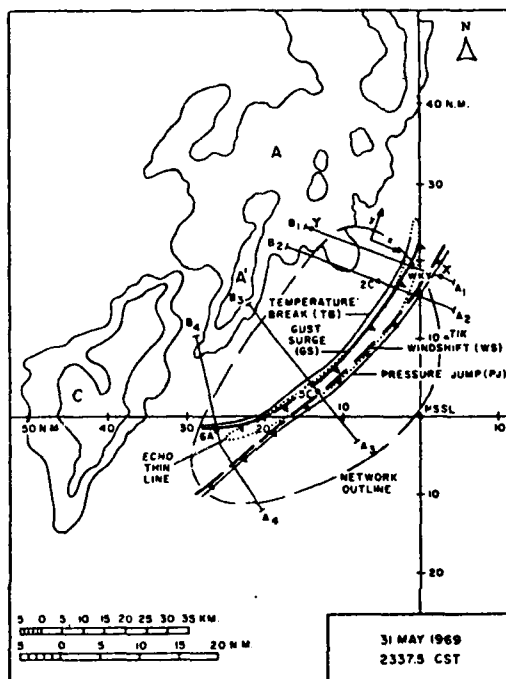
Fig. 3.17. Detailed structure of thunderstorm outflow, showing spatial relationship of outflow boundary to radar echo at a specific time (after Charba, 1974). Note the complex nature of the outflow boundary with the windshift line and pressure jump leading the temperature break and gust surge.
