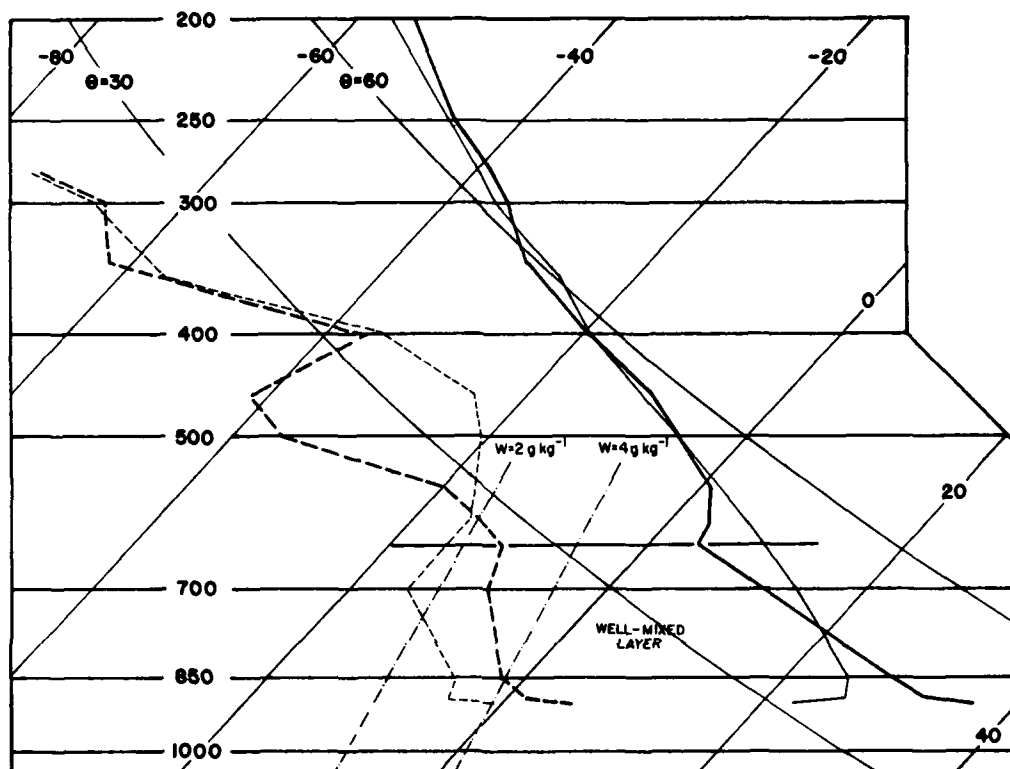
Fig. 3.12. Sample soundings through dry air on west side of dryline (Midland, Texas on 8 June 1974). Thin lines show temperature (solid) and dewpoint (dashed) curves at 1200 GMT. Thick lines show similar curves at the following 0000 GMT sounding time. Dash-dot lines show representative mixing ratio lines on the chart. Note shallow, surface superadiabatic "contact" layer at 0000 GMT.
