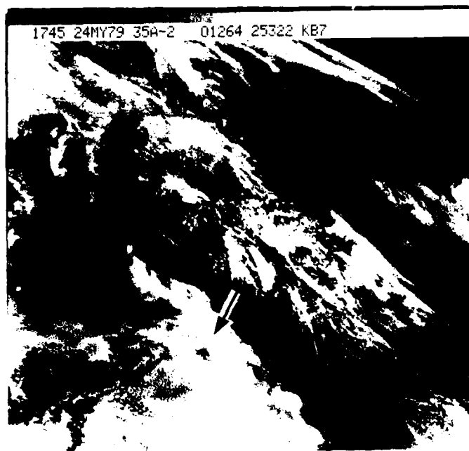
Fig. 3.37. Vortex trail revealed in wake of Guadalupe Island (arrow) in layer of stratocumulus clouds.
