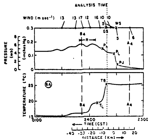
Fig. 3.19. Example of time sequence of events during gust front passage at a point (after Charba, 1974). See Fig. 3.17 for explanation of abbreviations.
