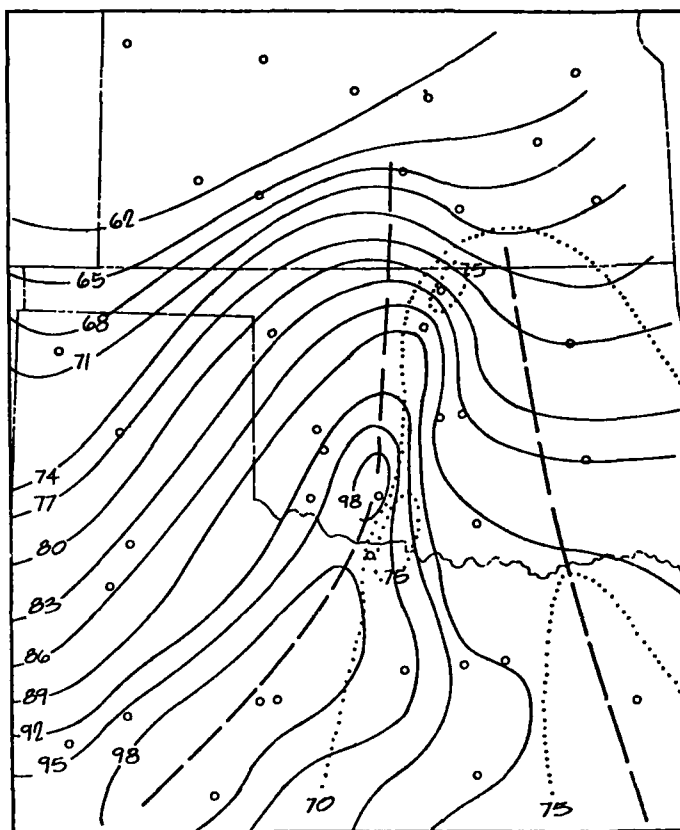
Fig. 3.30. Surface temperature and dewpoint (solid and dotted lines, respectively; °F) analysis at 1900 GMT, 8 June 1974 (after Moller, 1979). Thermal and moisture axes are shown as dashed lines, while open circles locate surface observation sites.
