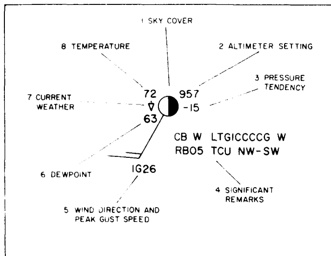
Fig. A.2. Station model for plotted surface observations. Note that the second digit of the wind direction is indicated - in this example, a wind from 310° and a "1" shown. Wind speeds are in kts, temperature in °F, altimeter setting in tenths of an inch of mercury (leading digit suppressed - in this example, 29.57 in Hg = 957) and 3-h pressure tendencies in tenths of a millibar (down 1.5 mb over past 3 h = -15).
