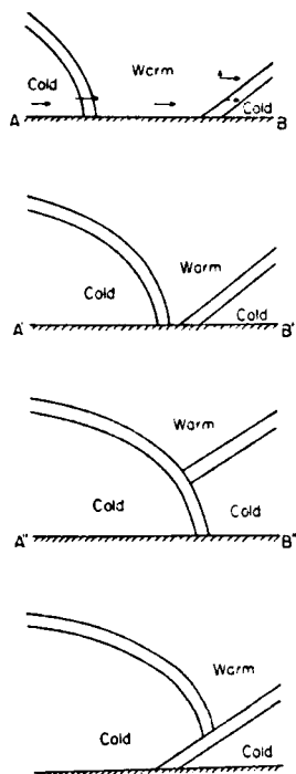
Fig. 3.10. Schematic example showing formation of an occluded front, with cold front overtaking warm front (after Saucier, 1955). In the example on the bottom, the cold air ahead of the warm front is colder than that behind the cold front, giving rise to a warm-type occlusion. This is relatively rare in the U.S. In the case just above, the cold air behind the cold front is colder than that ahead of the warm front, yielding a cold-type occlusion.
