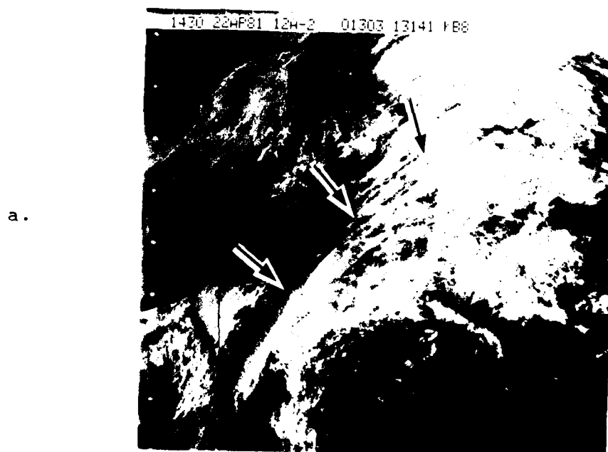
Fig. 2.7. Visible (a) and enhanced infrared (b, next page) satellite images showing anticyclonically curved band of cirrus across Texas, Oklahoma, southeastern Kansas and Missouri. Such bands are associated with upper level jet streams, with the jet axis from 1^\circ to 5^\circ poleward of the sharp cloud edge.
