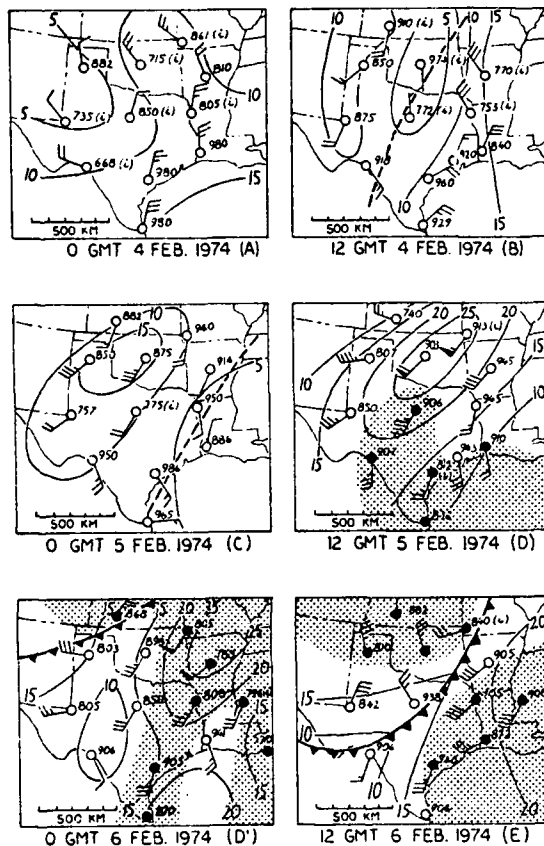
Fig. 3.34. Time evolution of a low level jet stream (after Djuric and Damiani, 1980). Winds shown are at the level of maximum wind in the lowest 2 km, isotachs are in m s^{-1} while relative humidities over 80% are stippled. The dashed line locates the ridge at 850 mb.
