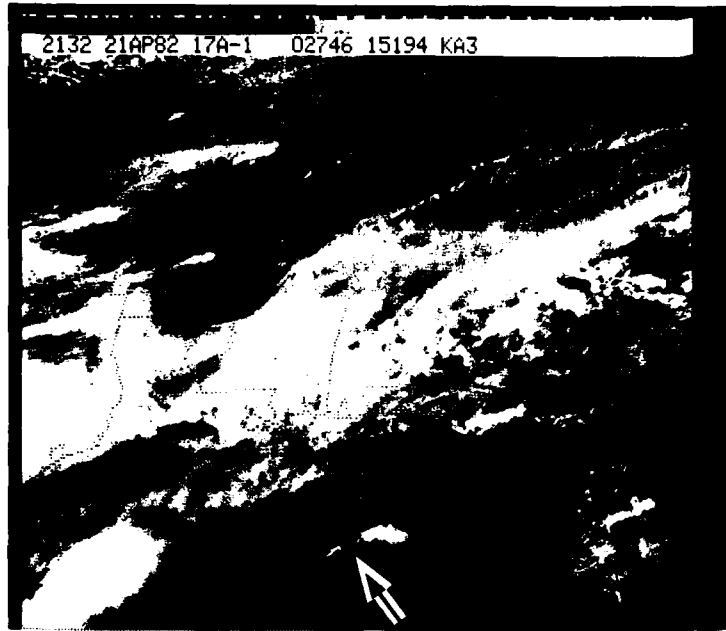
Fig. 3.23. Visible satellite image showing a small, nearly circular outflow boundary in the Gulf of Mexico (arrow). Note the ring of enhanced cumulus surrounding the area of nearly cloud free air. Remnants of the thunderstorm anvil can be seen on the northeast side of the ring.
