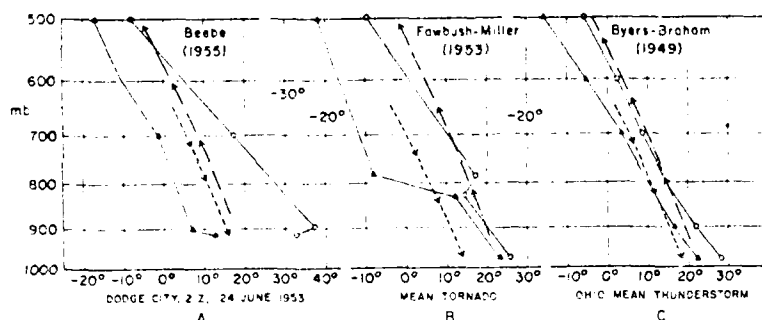
Fig. 2.9. Schematic of three distinctive soundings associated with severe convection in the U.S. (after Newton, 1980). Type A is an "inverted T" sounding typical of the High Plains or desert severe storms. Type B is the classical "loaded gun" sounding characteristic of Great Plains or central U.S. severe weather outbreaks. Type C is common over Gulf coastal states and in summer east of the Mississippi River. Dash-dotted lines correspond to moist adiabats associated with low-levels and dashed lines to moist adiabats in lower middle levels (1000-700 mb).
