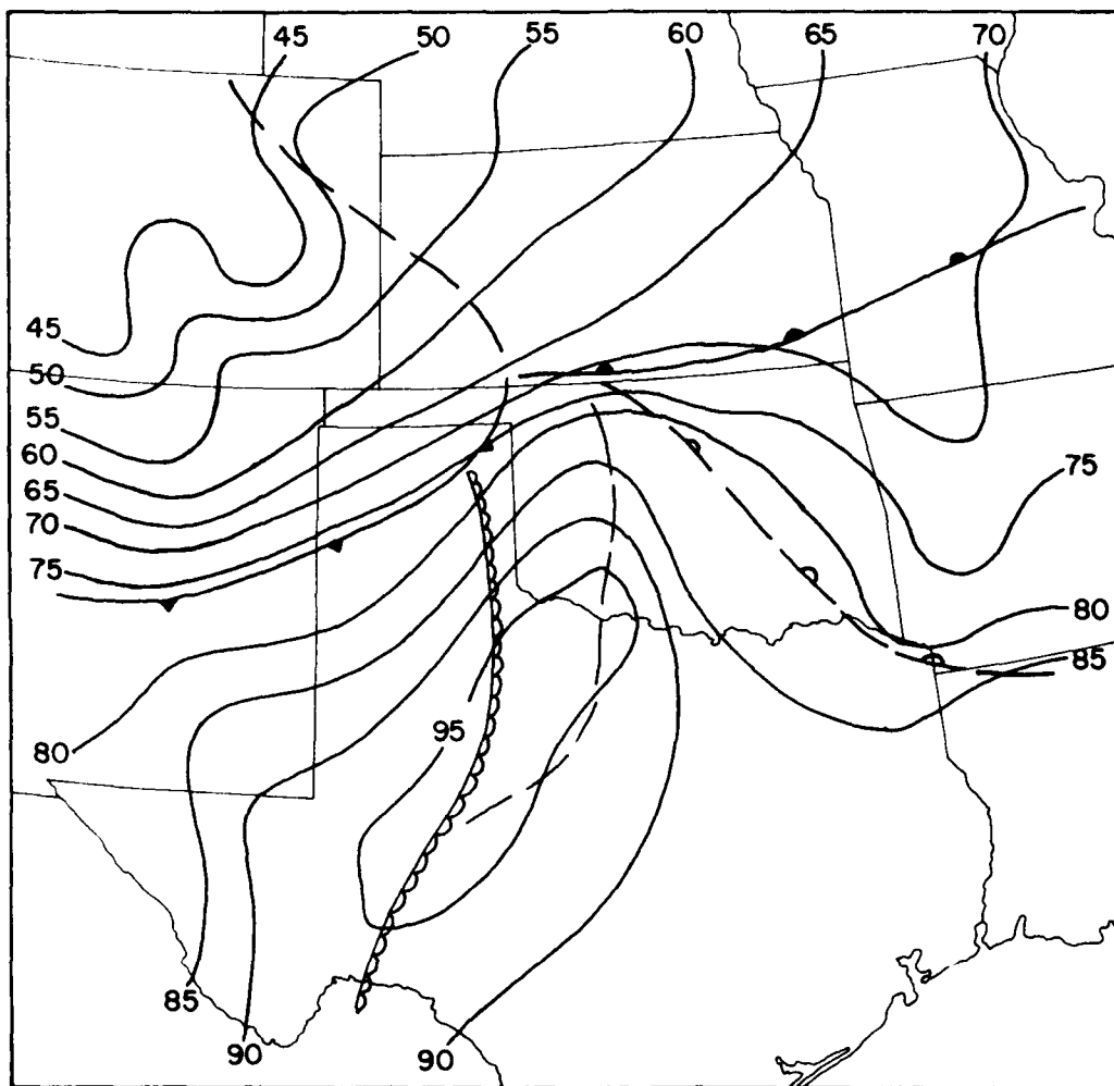
Fig. 3.3. Isotherms ( ^{\circ}\text{F} ) and one possible frontal analysis for data in Fig. 3.2.
