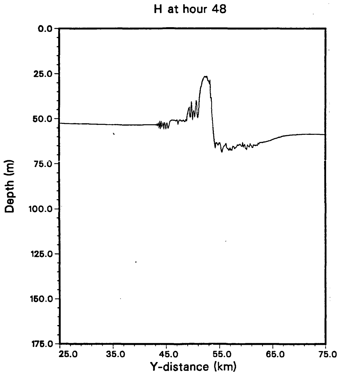
Figure 14. Frnt 1 Case II 48-Hour Mixed Layer Depth.
