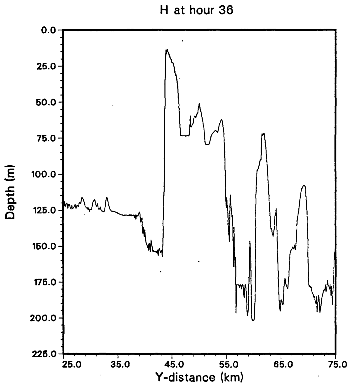
Figure 26. Frcnt 2 Case I 36-Hour Mixed Layer Depth.
