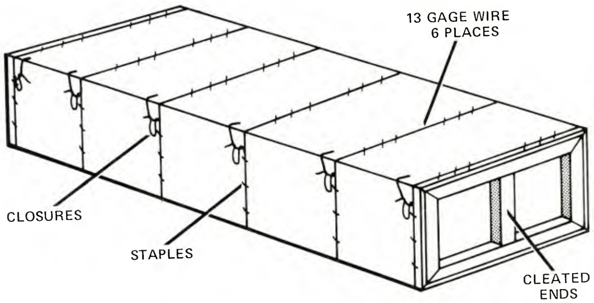
Figure 4. Wirebound box
