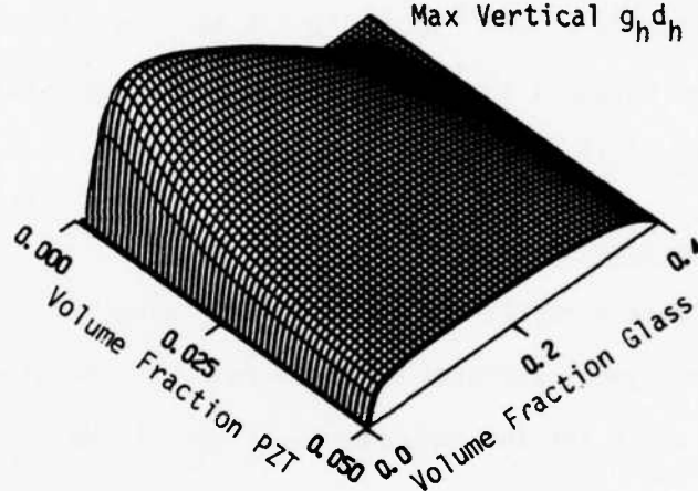
Figure 3.6. PZT:glass:polyurethane 1:2:3 composite.
