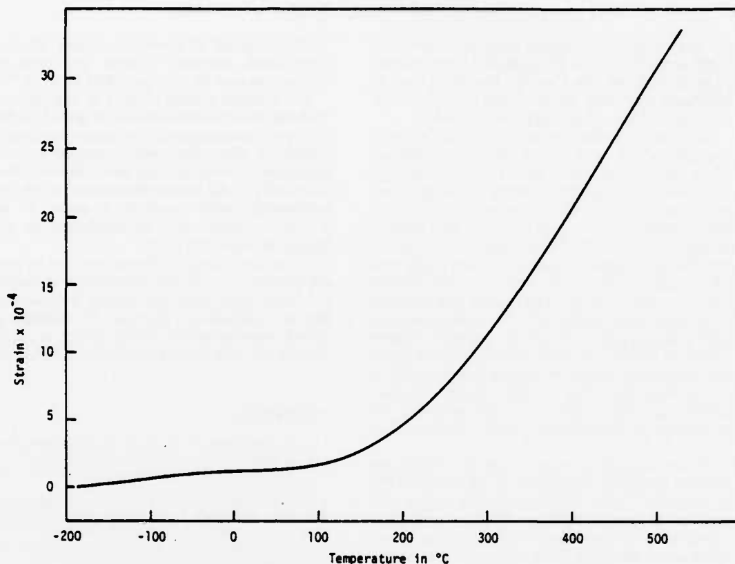
FIGURE 3 Thermal strain of polycrystalline 0.9 PMN-0.1 PT ceramic. The linear thermal expansion is about 10^{-5} \text{ } ^\circ\text{C}^{-1} at 400^\circ\text{C} and less than 10^{-6} \text{ } ^\circ\text{C}^{-1} at room temperature.
