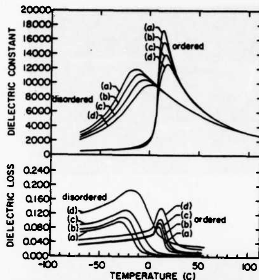
FIG. 4. Temperature dependence of dielectric constant and dielectric loss of ordered ( S = 0.80 ) and disordered ( S = 0.35 ) single crystals at (a) 1 kHz, (b) 10 kHz, (c) 100 kHz, (d) 1000 kHz.
