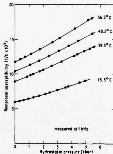
Figure 4 Hydrostatic pressure dependence of the reciprocal permittivity in \text{Pb}(\text{Mg}_{1/3}\text{Nb}_{2/3})\text{O}_3 at various temperatures.
