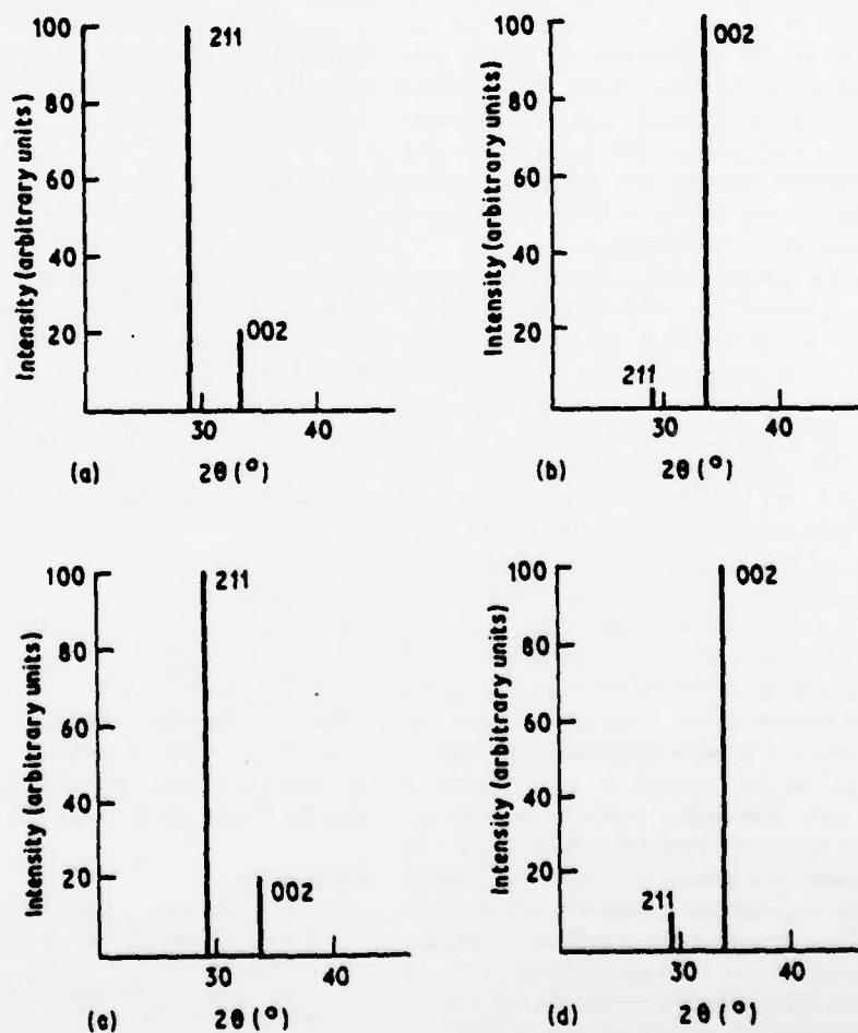
Figure 4 X-ray diffraction patterns of (a) \text{Ba}_2\text{Ge}_2\text{TiO}_7 , standard powder diffraction pattern, (b) BTG glass-ceramic, (c) \text{Ba}_2\text{TiSi}_2\text{O}_7 , standard powder diffraction pattern, and (d) BTS glass-ceramic.
