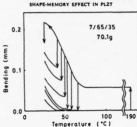
FIGURE 8 Reduction of bending by removal of the load at different temperatures in the sample 7.0/65/35.
