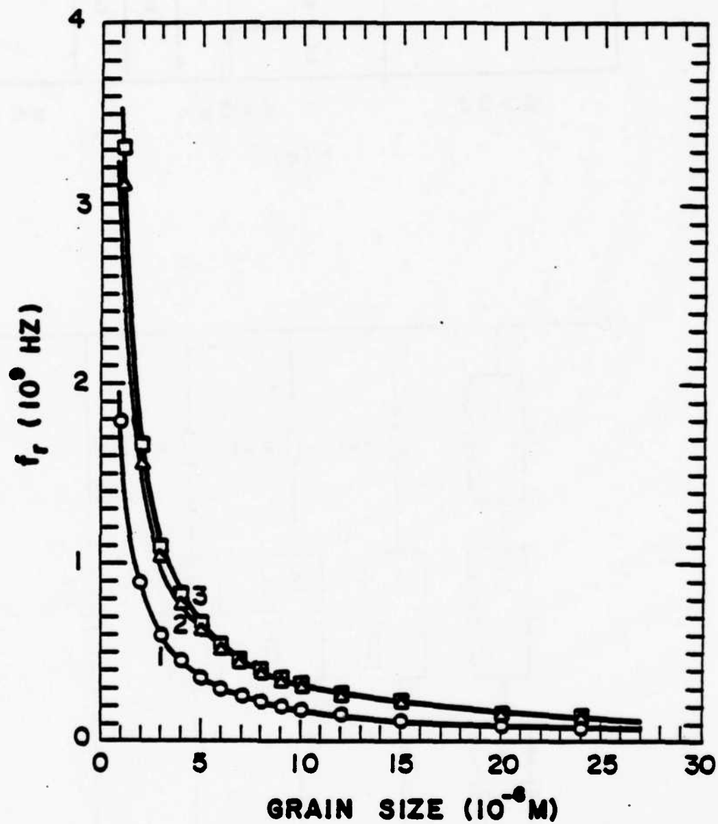
Resonant frequency of \text{LiNbO}_3 single cube-shaped grain.
