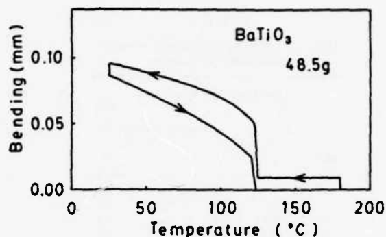
FIGURE 6 Temperature-dependence of bending of \text{BaTiO}_3 .
