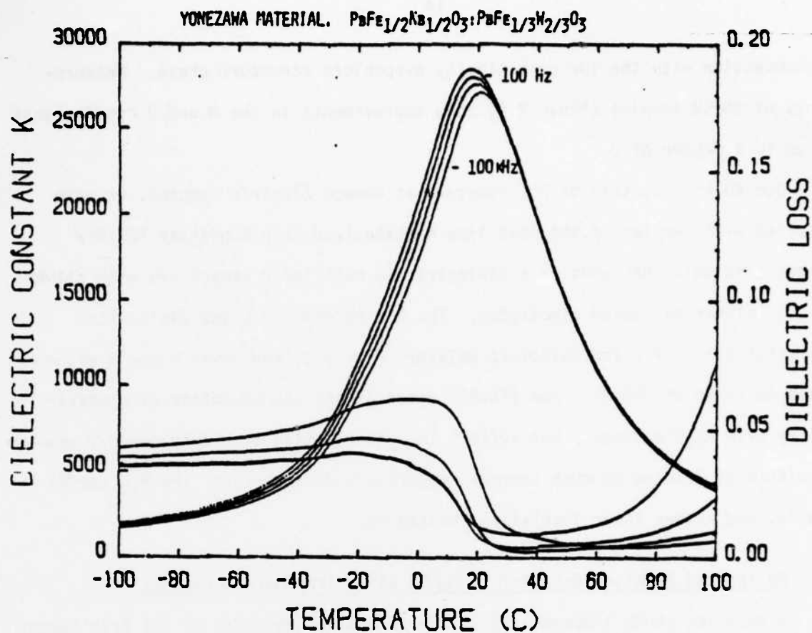
Figure 2.5. Dielectric behavior of typical PFeN:PFeW ceramic.
