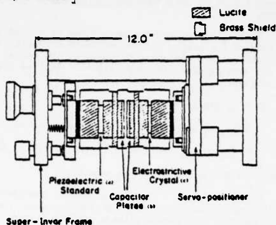
Sample Holder
