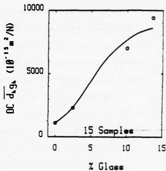
Figure 3.2. Experimental data PZT:Devcon.
