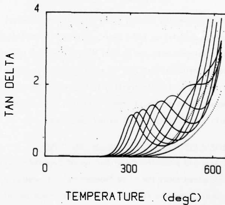
Figure 7.4. Tangents delta in PLZT 8.6:30:20 + 0.05% Mn.
