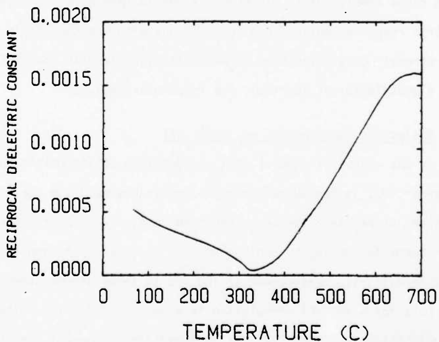
Figure 7.2. Dielectric stiffness vs T in PZT 501 (10 kHz).
