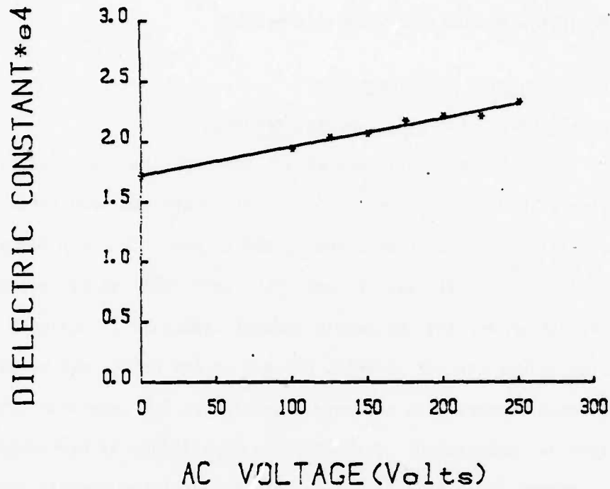
Figure 2.3. \epsilon vs V in PMN:10% PT.
