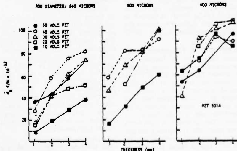
Fig. 11 \bar{d}_h as a function of volume % PZT, rod diameter and composite thickness.
