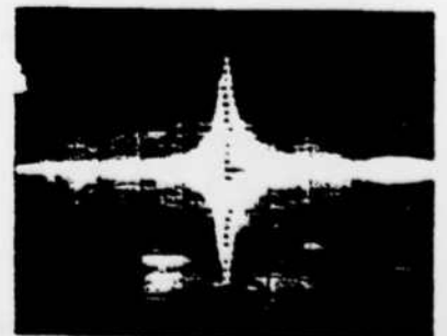
Fig. 20(a) Bandwidth broadening in parallel connected resonant composites. (a) Q=2^0 .
