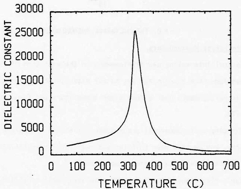
Figure 7.1. Dielectric permittivity vs T in PZT 501 (10 kHz).
