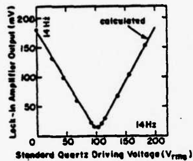
Fig. 13 Null condition method between PMN and quartz.
