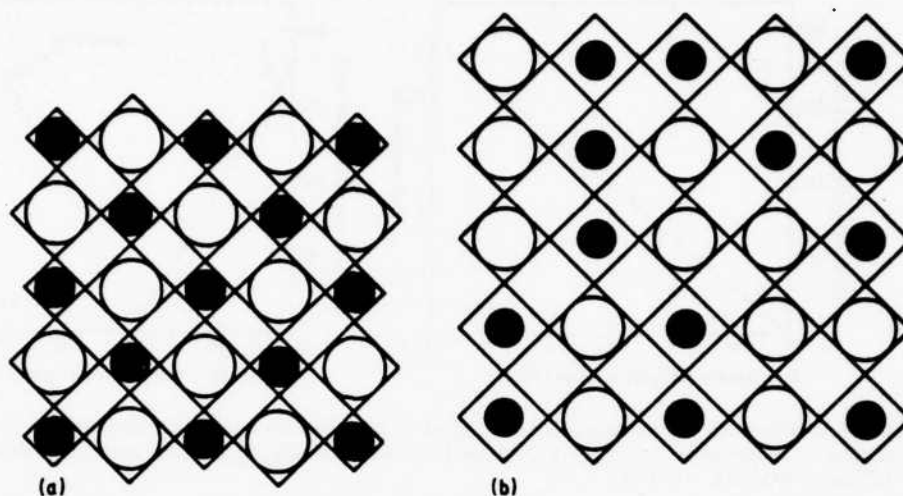
Figure 7 Crystal structure models of the A(B_{1/2}B_{1/2})O_3 type perovskite: (a) ordered structure with a small rattling space, and (b) disordered structure with a large rattling space. \circ = B_I ion and \bullet = B_{II} ion.
