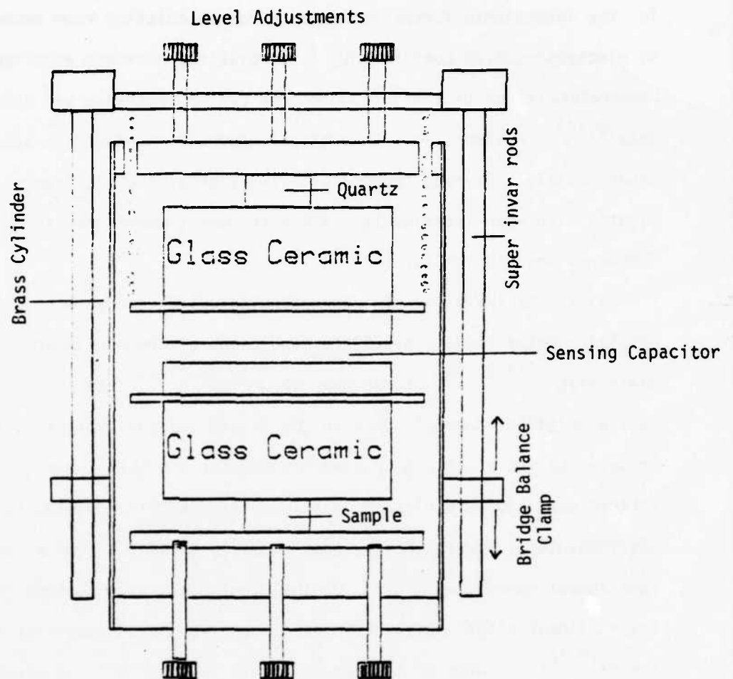
Figure 2.2. Sample holder for AC dilatometer showing Invar: Brass bridge for expansion balance.
