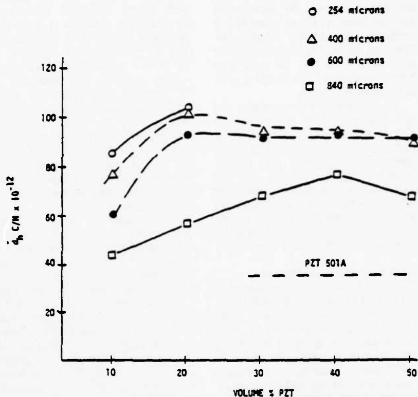
Fig. 12 \bar{d}_h as a function of volume % PZT and rod diameter (sample thickness 4 mm).
