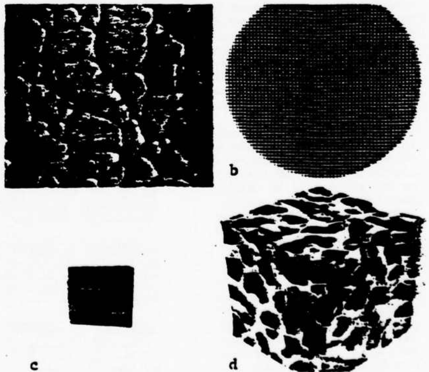
Fig. 4 Four types of connectivity: (1) 3-0, (b) 3-1, (c) 2-2 and (d) 3-3 (replamine).
