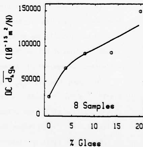
Figure 3.4. Experimental data epoxy reinforced PZT:Devcon:foam.
