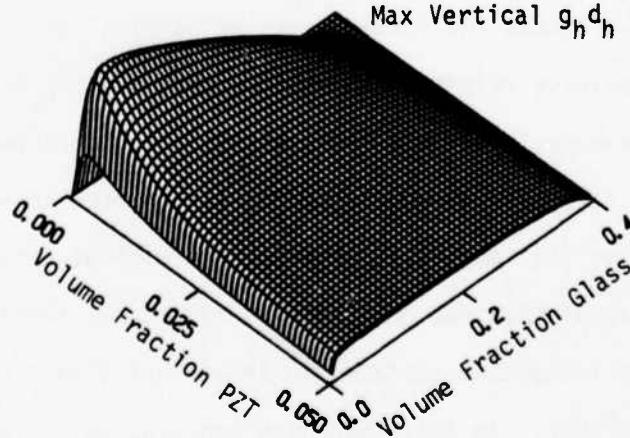
Figure 3.7. PZT:glass:polyurethane foam 1:2:3:0 composite 20 vol% foaming.
