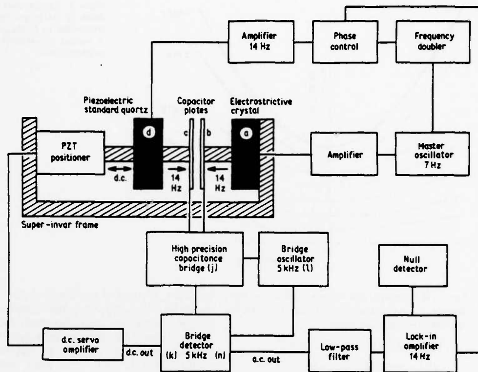
Figure 5 Schematic diagram of the a.c. capacitance dilatometer.
