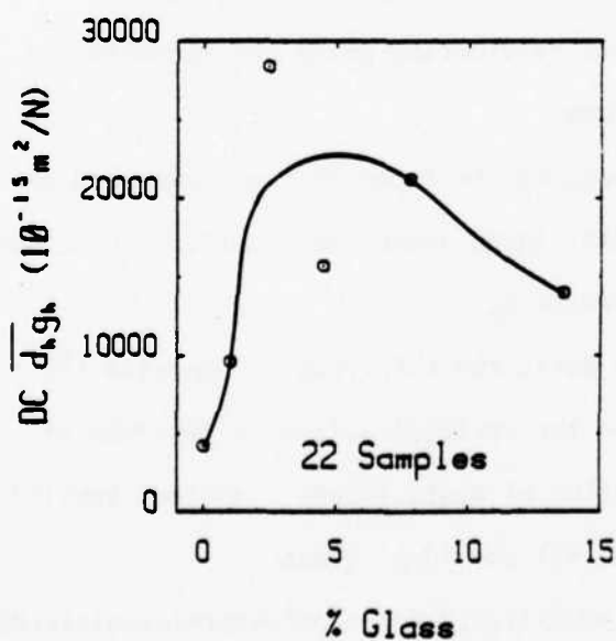
Figure 3.3. Experimental data PZT:Devcon:foam.
