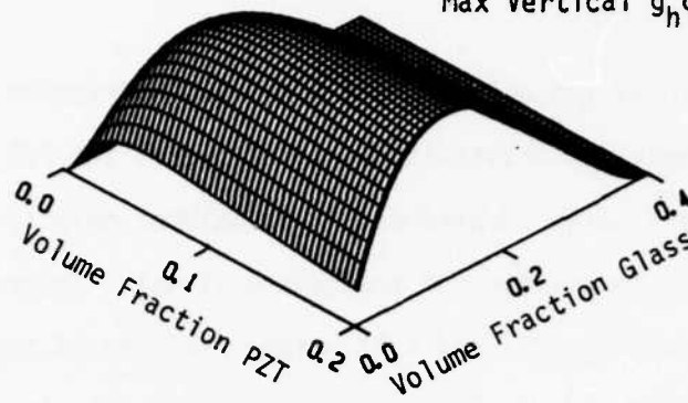
Figure 3.5. PZT:epoxy composite.
