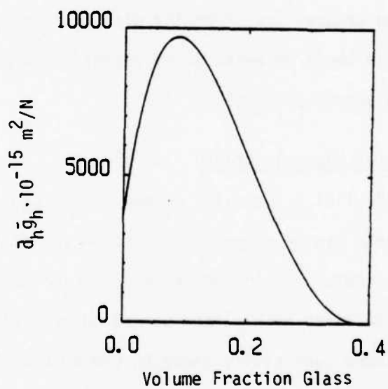
Figure 3.9. Theory for 5% PZT (Expanded Scale).
