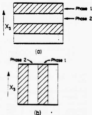
Fig. 6 The series (a) and parallel (b) models used in estimating the piezoelectric and pyroelectric effects of diphasic solids.
