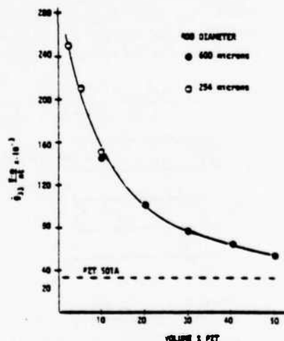
Fig. 10 \bar{g}_{33} as a function of volume % PZT.
