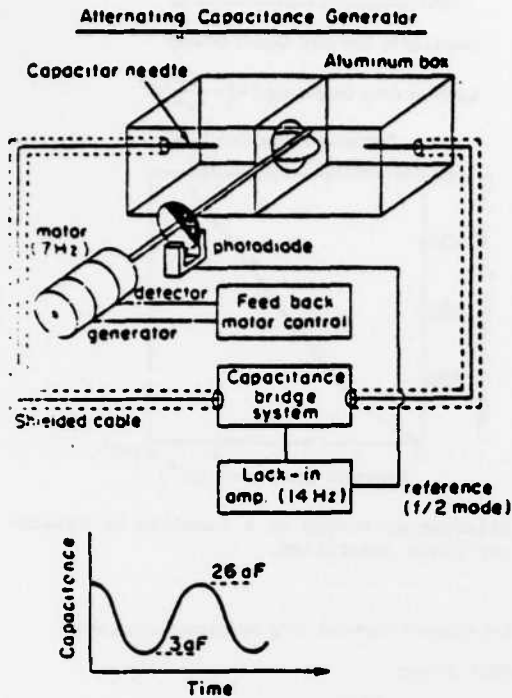
Fig. 9 Scheme of the alternating capacitance generator.
