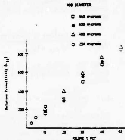
Fig. 9 Relative permittivity as a function of volume % PZT.
