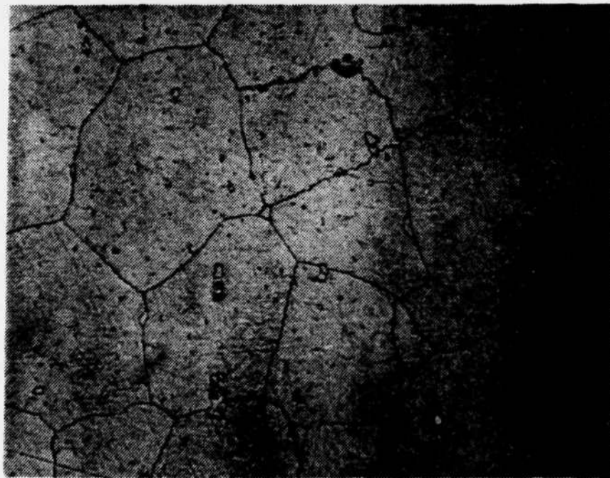
Fig. 4 Sample C Austenitized at 1200°C for thirty minutes. Magnification 250X
