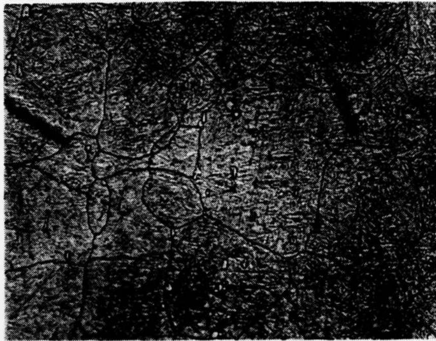
Fig. 5 Sample D Austenitized at 1180°C for thirty minutes. Magnification 250X
