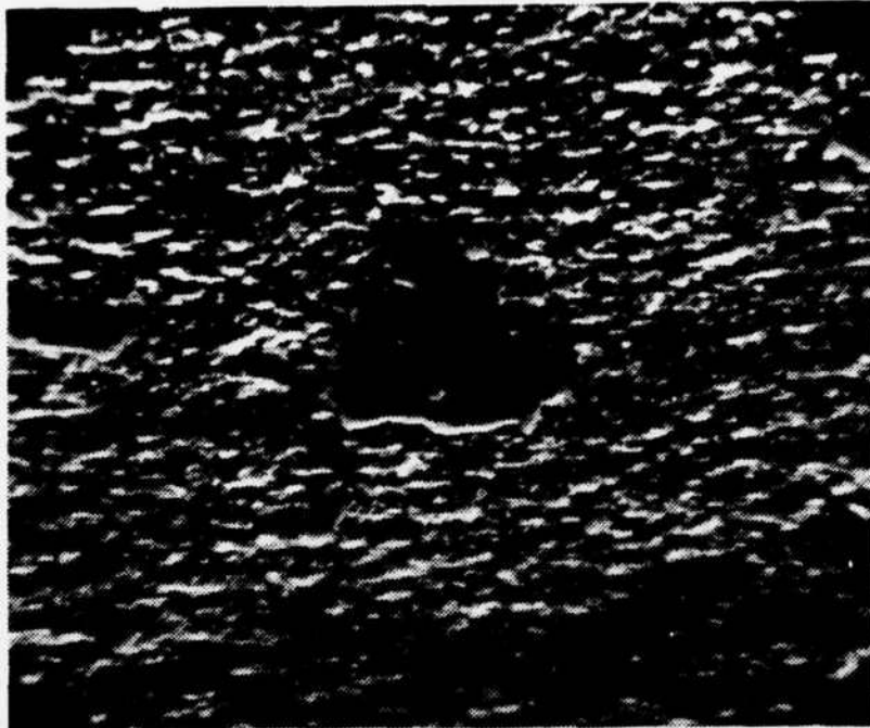
Fig. 9 Sample H Austenitized at 1150°C for five hours, warm-rolled at 700°C. Residual carbide on a background of finely dispersed temper carbides. Magnification 2200X
