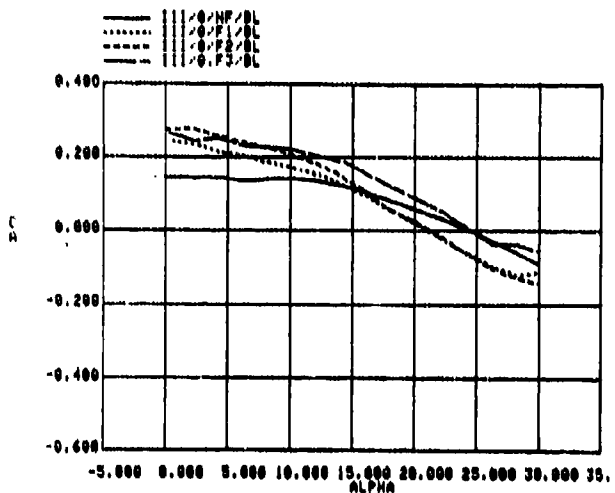
FIGURE A-13.2 FIN EFFECTS
