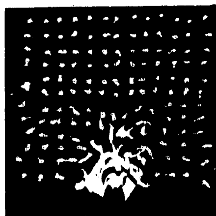
18d. MISSILE 111, 33^\circ ROLL, 20^\circ PITCH
