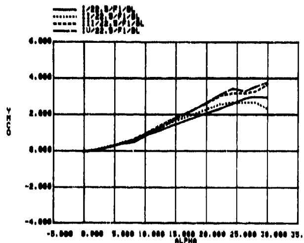
FIGURE A-5.6 BODY CORNER RADIUS EFFECTS
