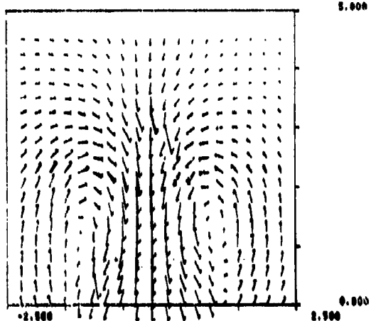
MISSILE 2, ROLL 0, ALPHA 30
