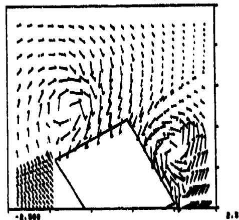
MISSILE 1, ROLL 33, BLNT HOS, ALPHA 25
