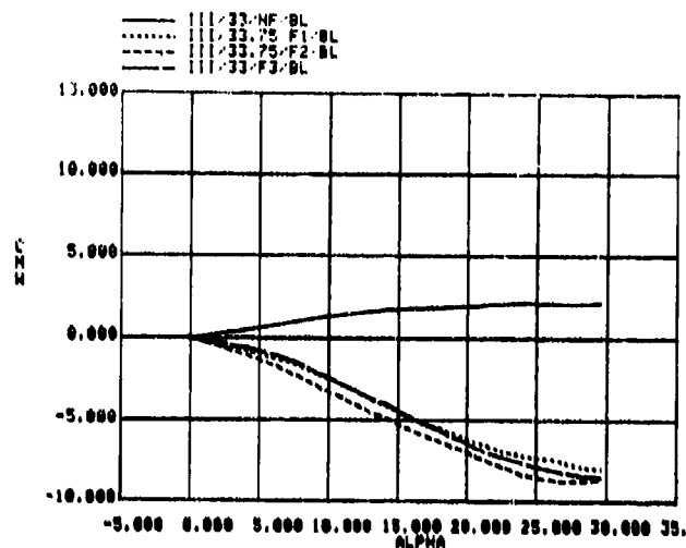
FIGURE A-28.4 FIN EFFECTS
