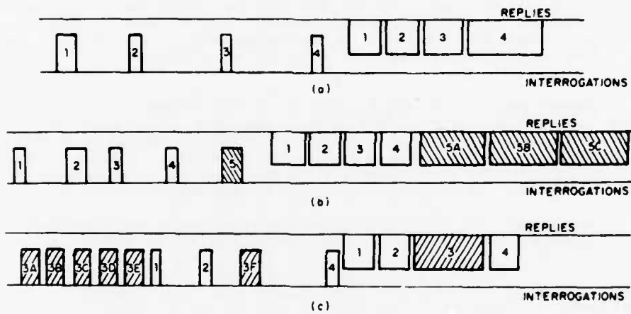
Fig. 3-4. Mode S cycles.
