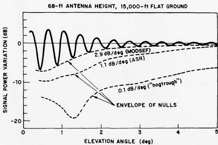
Fig. 5-1. Vertical lobing.
