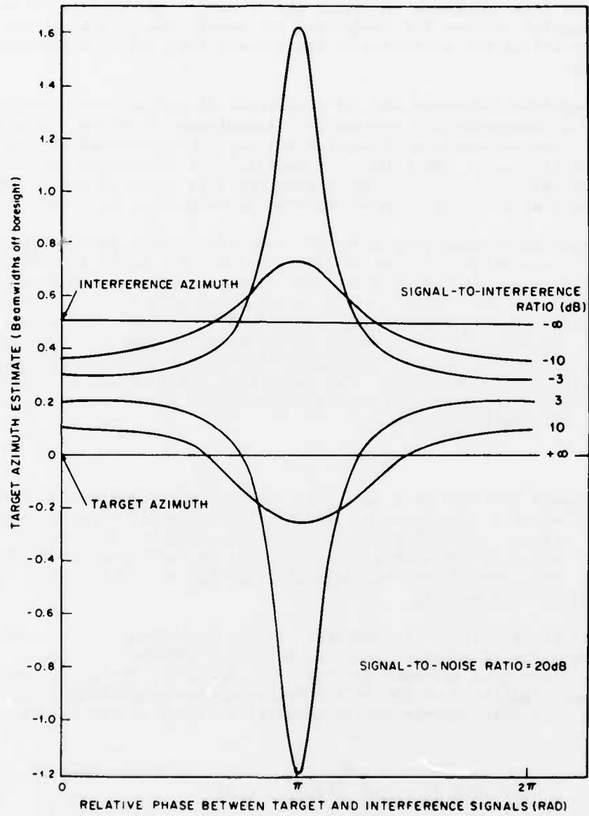
Fig. 5-6. Monopulse Estimate With Interference.
