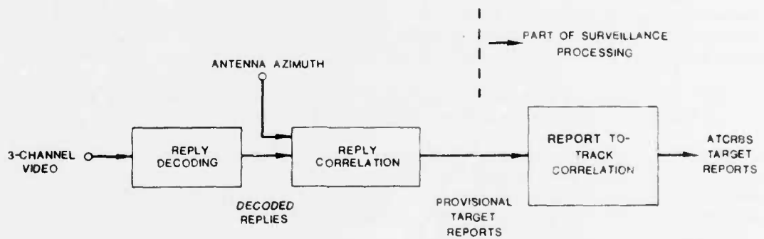
Fig. 3-12. ATCRBS reply processing.
