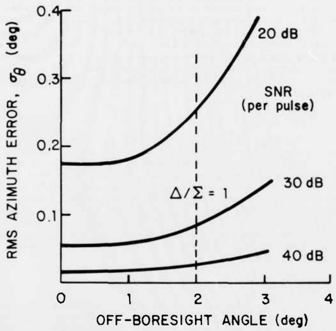
Fig. 5-5. Noise induced monopulse error.
