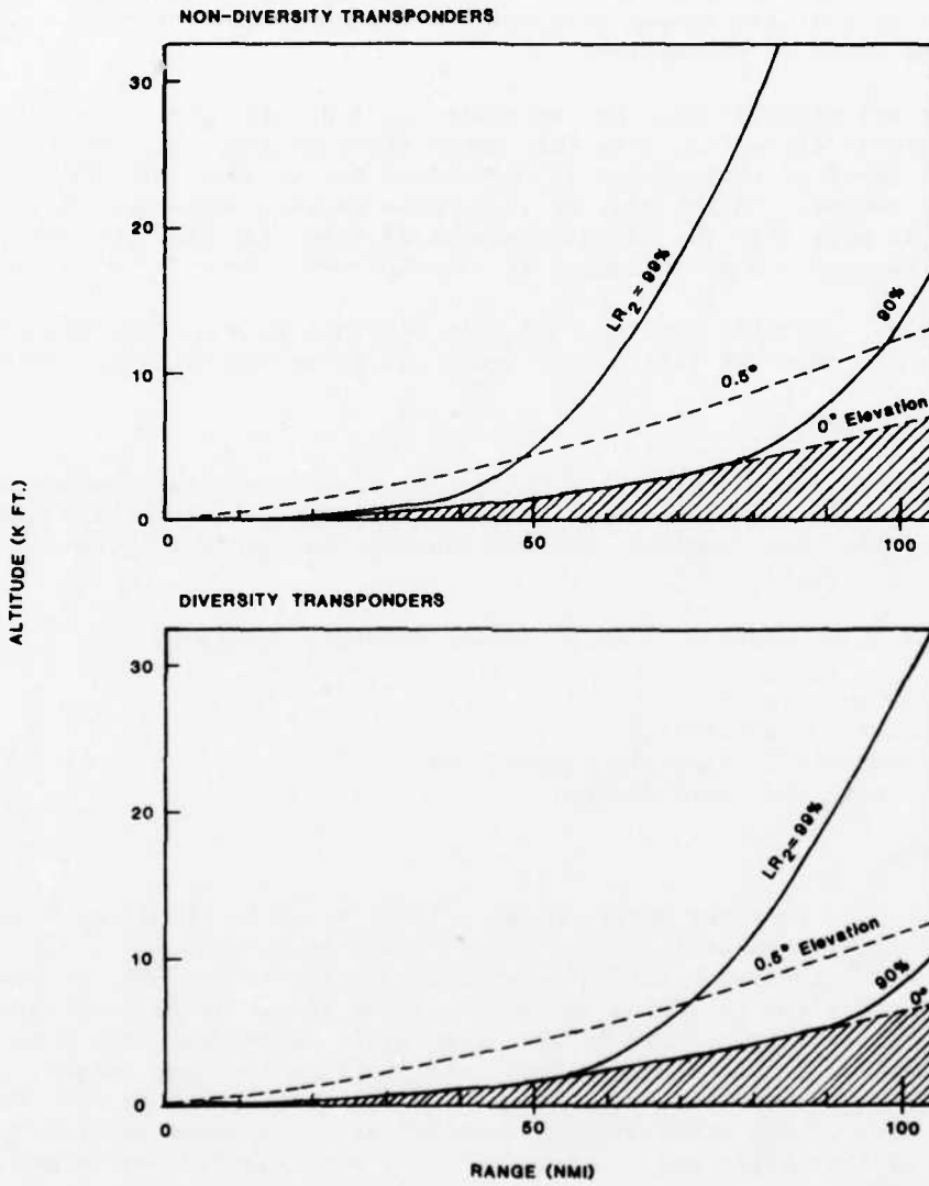
Fig. 5-4. Mode S link reliability for a terminal ground station.
