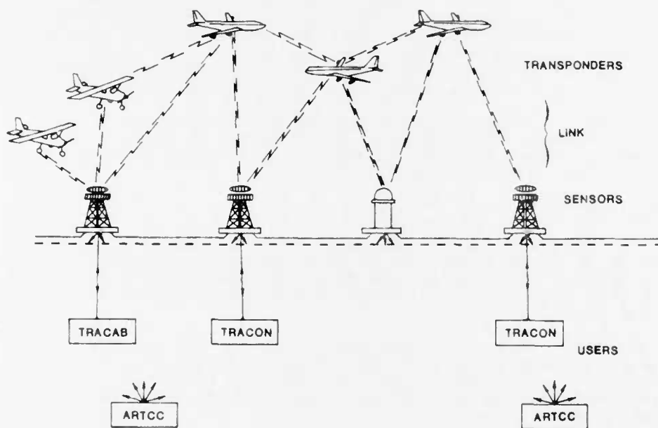
Fig. 1-2. Mode S system elements.
