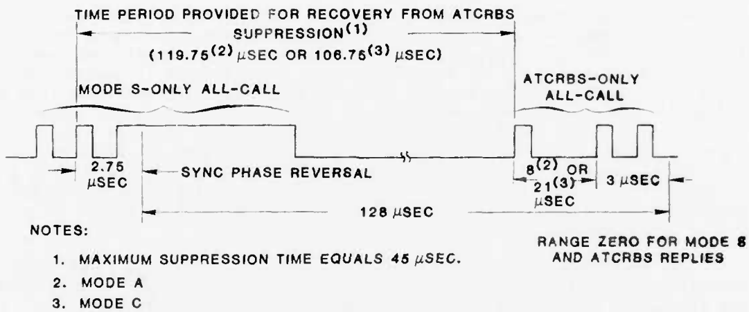
Fig. 2-8. Combined interrogation for site selective acquisition.
