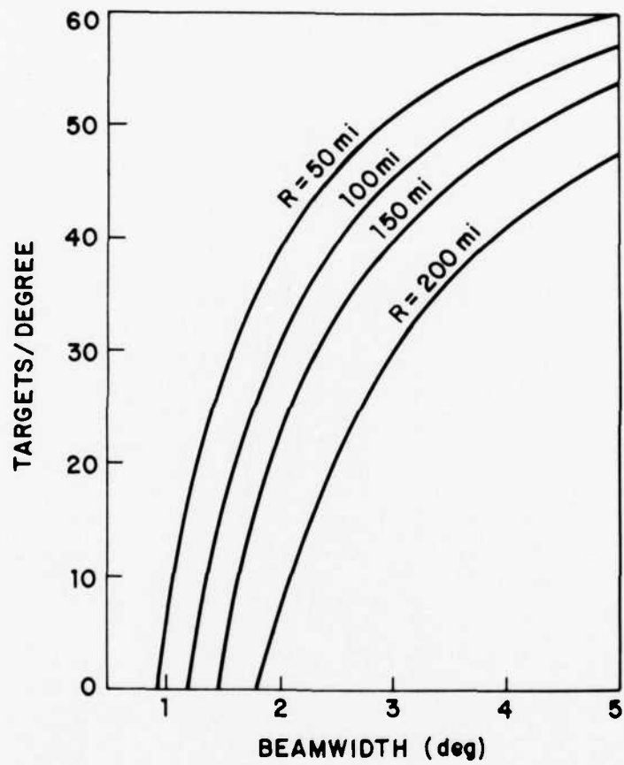
Fig. 5-8. Capacity plots.
