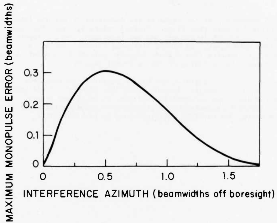
Fig. 5-7. Maximum monopulse error with target on boresight.
