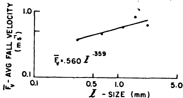
Fig. 17 Class-averaged-fall velocities from 1030 to 1035 EST on 12 Dec 82.
