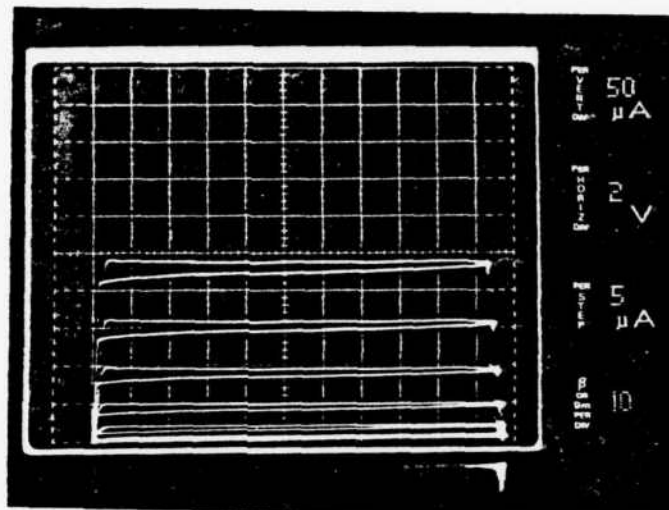
FIGURE 4.12d Second Set PSF/Epitaxy Transistor I_c - V_{ce} Characteristics
