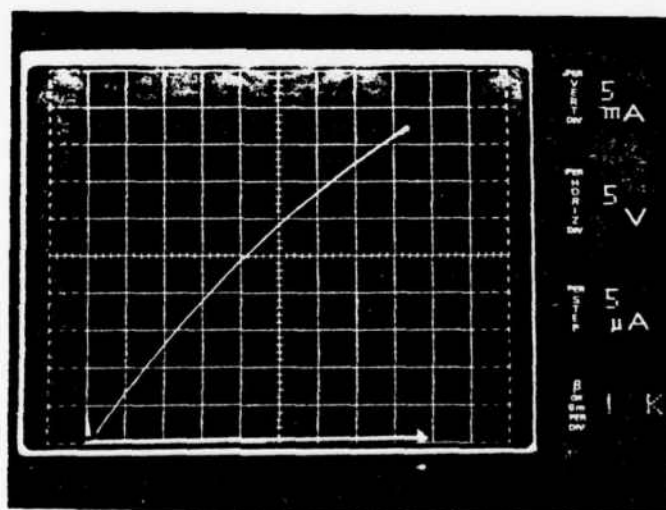
FIGURE 4.12e Second Set PSF/Epitaxy Transistor
