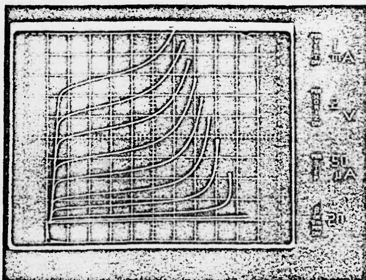
Figure 4.8. MOSBJT (epitaxial base) reverse BJT characteristics. Gate oxide is 10,000Å.
