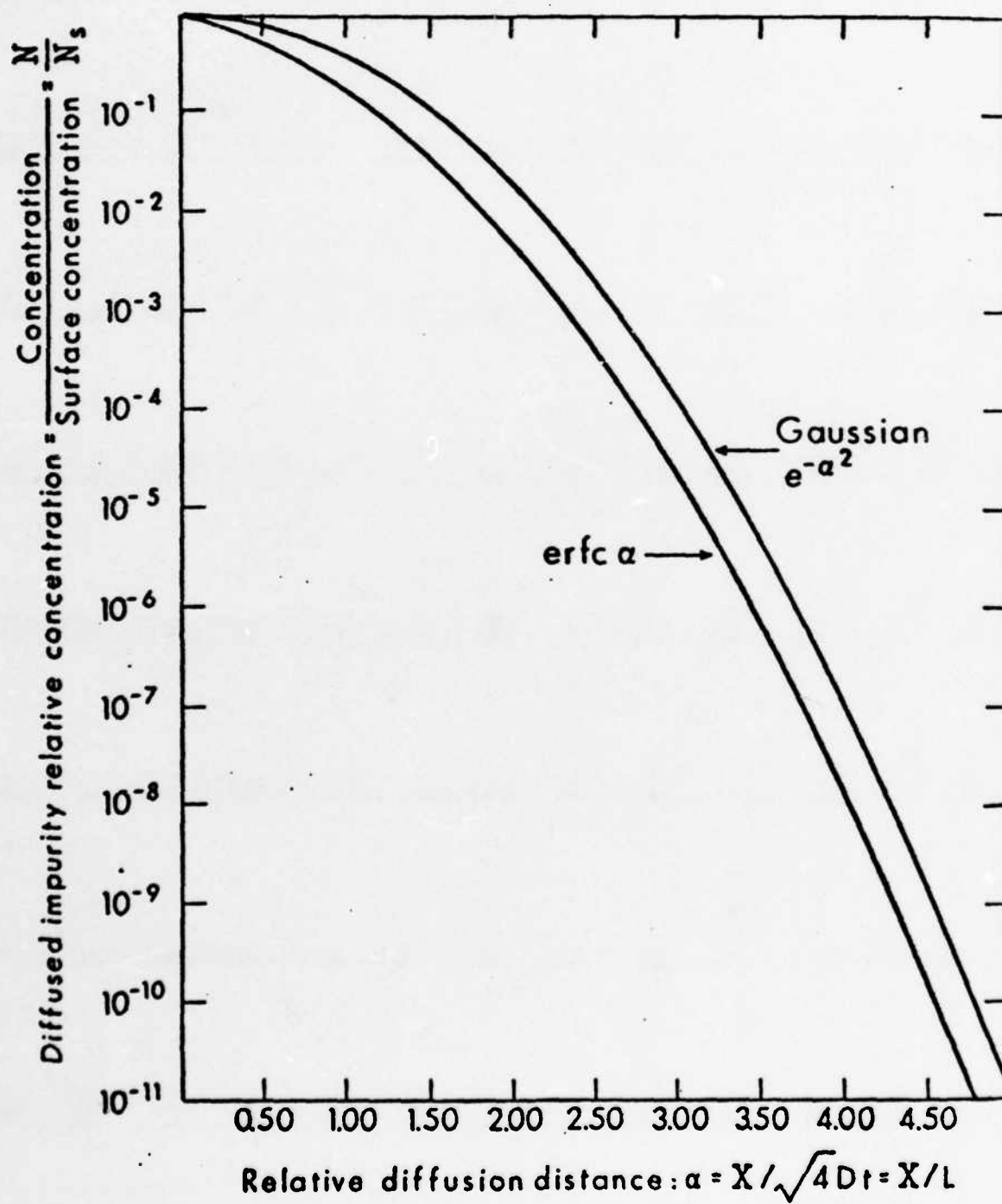
Figure 3.9. Normalized curves for erfc \alpha and e^{-\alpha^2} .
