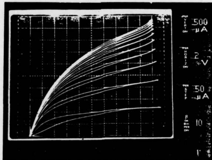
Fig. 3.2b The rectangular MOSBJT I_D/I_C - V_{DE}/V_{CE} characteristics V_G=20V , \Delta I_B=50.0 \mu A
