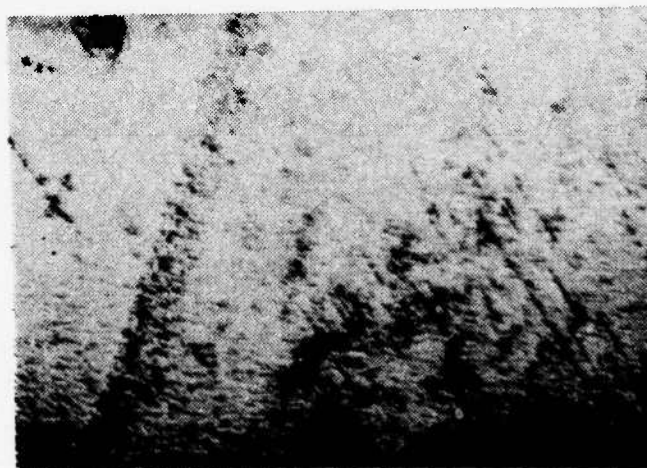
Figure 21. Alloy D (15 thermal cycles). A continuation of Figure 20 shows the concentration of dislocations to a distinct region of the matrix. (20,000X)
