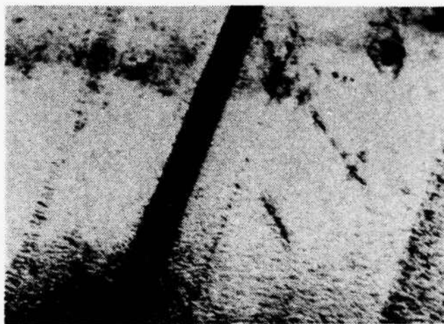
Figure 20. Alloy D (15 thermal cycles). Dislocations have a distinct angular relationship with vestigial structures. (20,000X)
