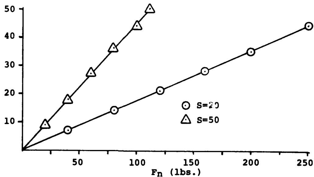
Fig. A.3 - Calibration of Kistler dynamometer in F_n direction.
