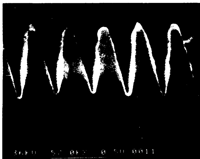
Fig. 35. SEM Photograph of Grating #8 Showing Grating Profile Horizontal Line Equals 0.5 \mu\text{m}
