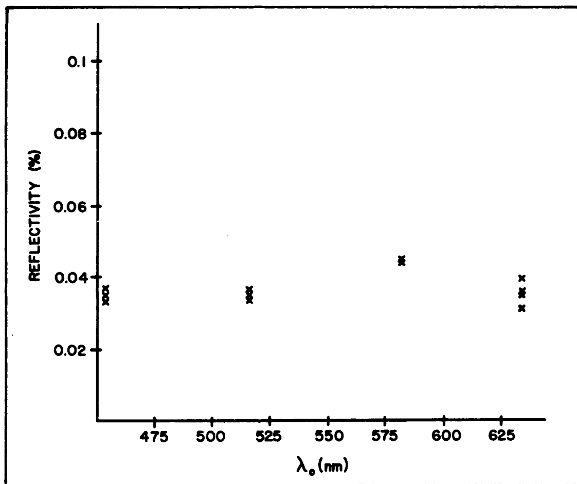
Fig. 36. Reflectivity of Grating #5 In Percent vs. Wavelength (Measured At Normal Incidence) X's Indicate Each of Several Measurements
