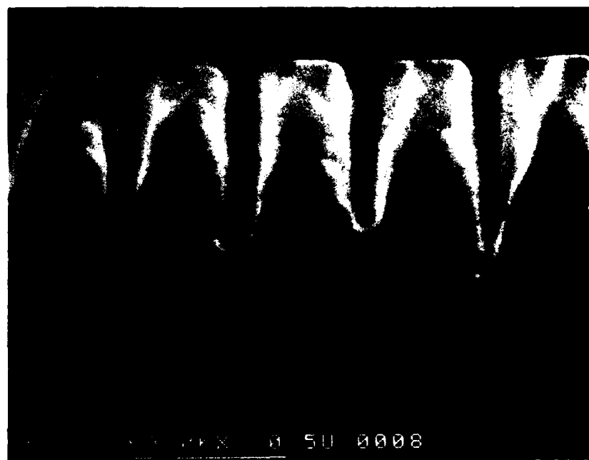
Fig. 33. SEM Photograph of Grating #3 Showing Grating Profile Horizontal Line Equals 0.5 \mu\text{m}
