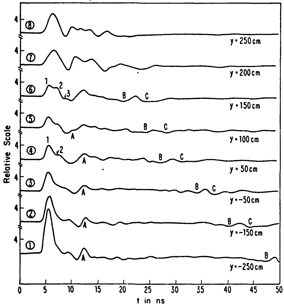
Figure 17. Vertical electric-field pulse sequences measured along centerline ( x = z = 0 ) of ground plane in Harvard model simulator; R_L = 90 \Omega .
