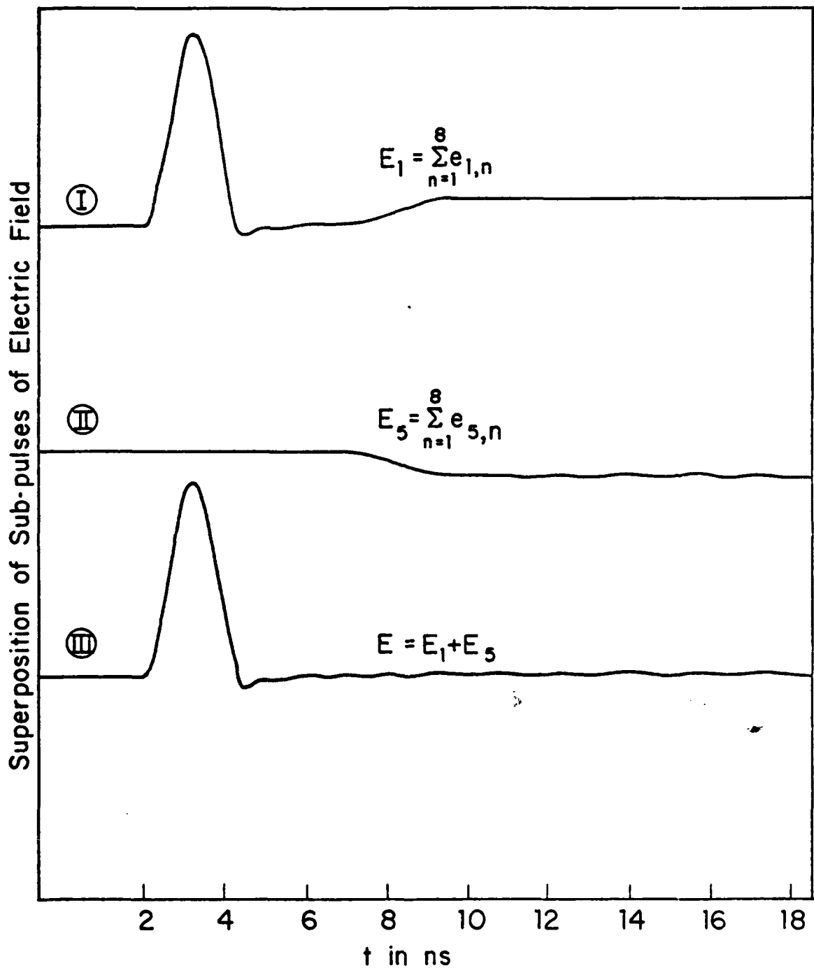
Figure 14. Superposition of subpulses of electric field at center of ground plane ( y=0 ) in rhombic simulator originating from: (I) front, (II) rear, and (III) all rhombic wires.
