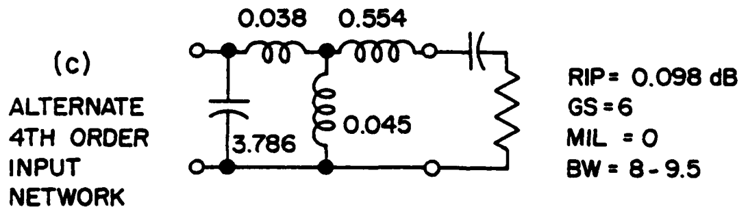
Figure 2.29. Power Amplifier Input Networks
