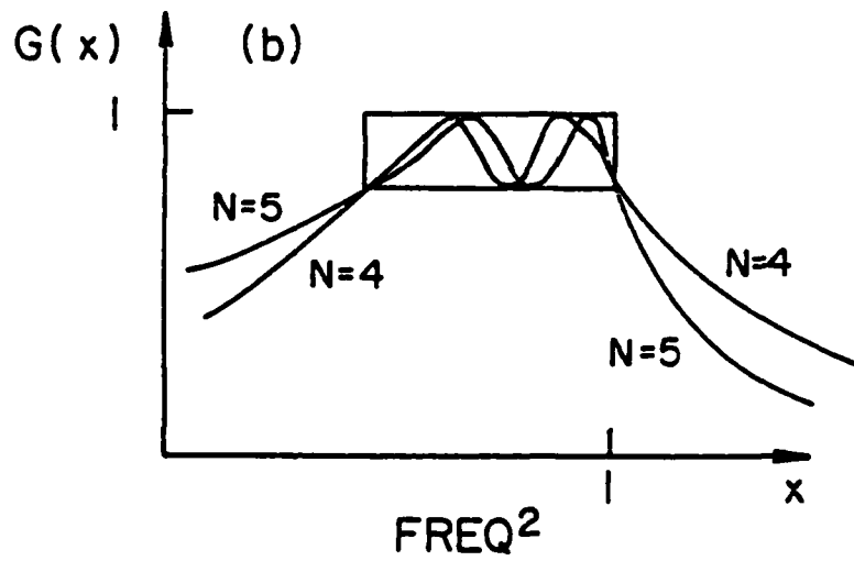
Figure 2.11. Gain Responses Outside the Passband
