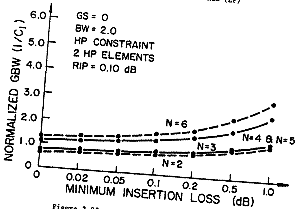
Figure 2.22. Gain-Bandwidth vs MIL (HP)
