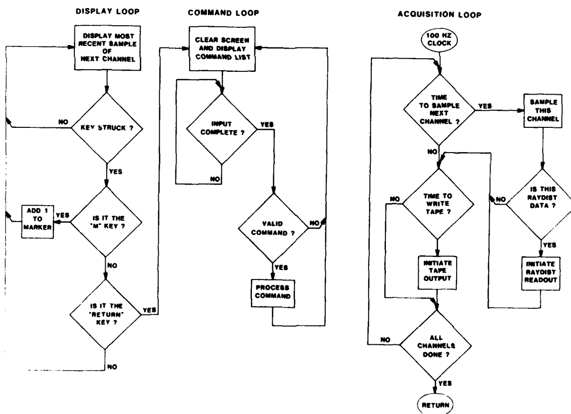
FIGURE 3. Simplified data acquisition software flowchart.
