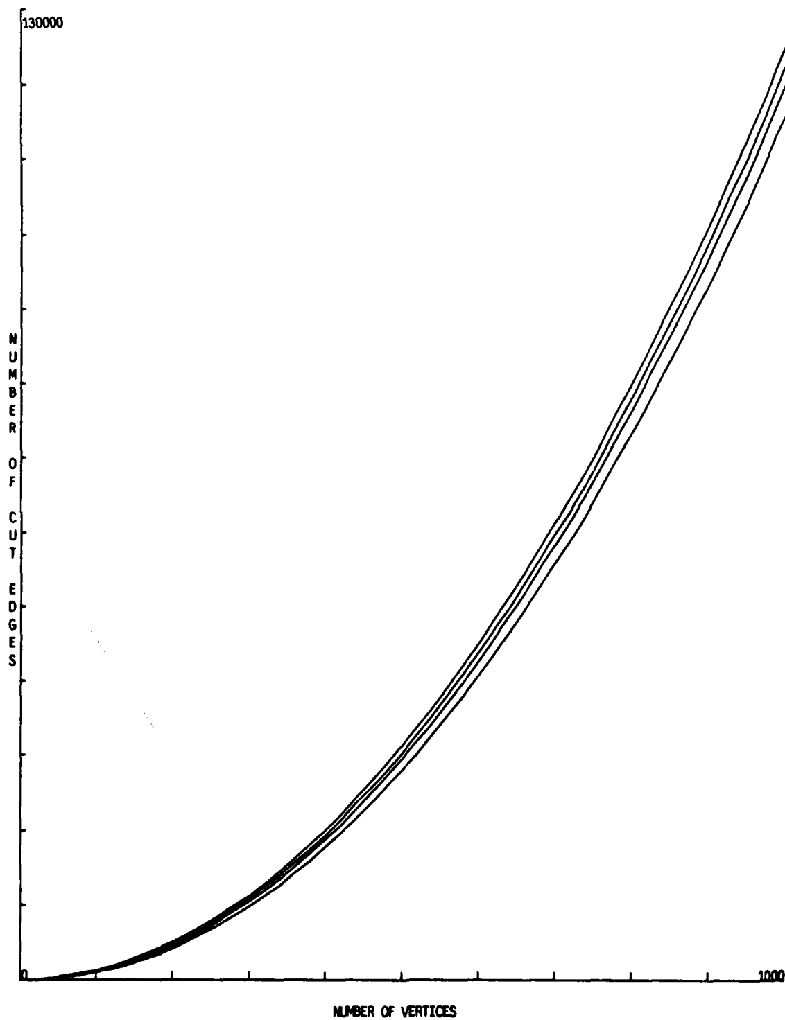
Figure 4.3. Graph of Vertex Size vs. Bisection Sizes
