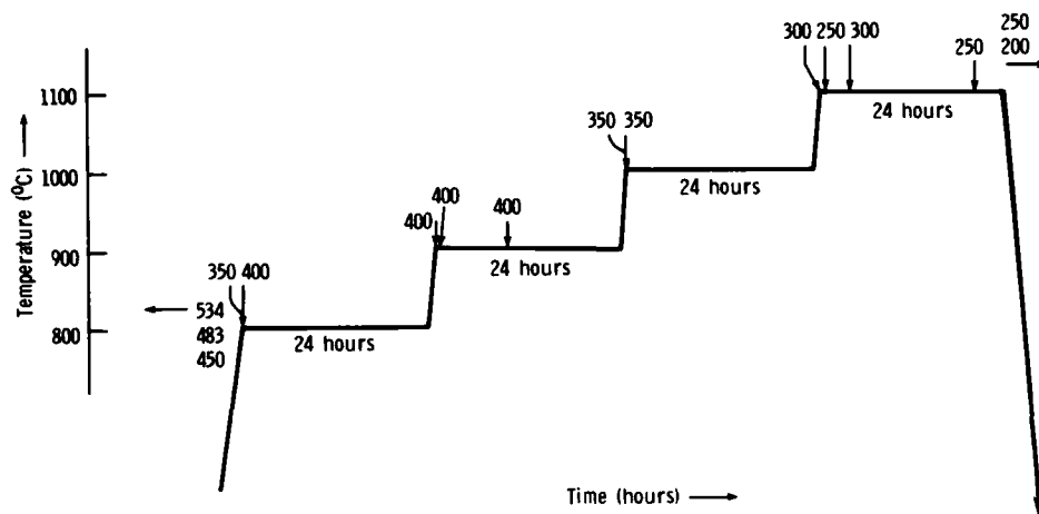
Figure 12. STSR results for CD hot-pressed silicon nitride.
