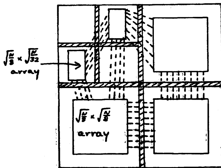
Figure 19. Another distribution of live cells which requires a wide center channel.
