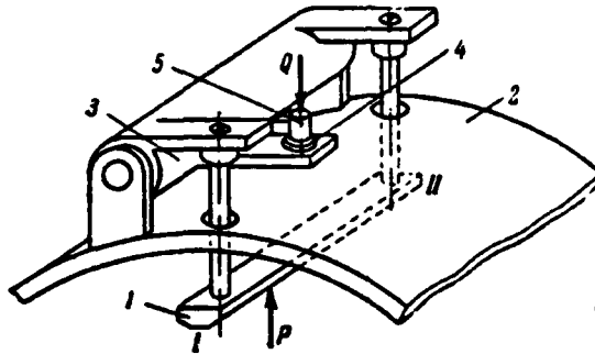
Fig. 66. The sensor, which is determining the values of the effort/force the point of application of which can be moved along line I-II.
