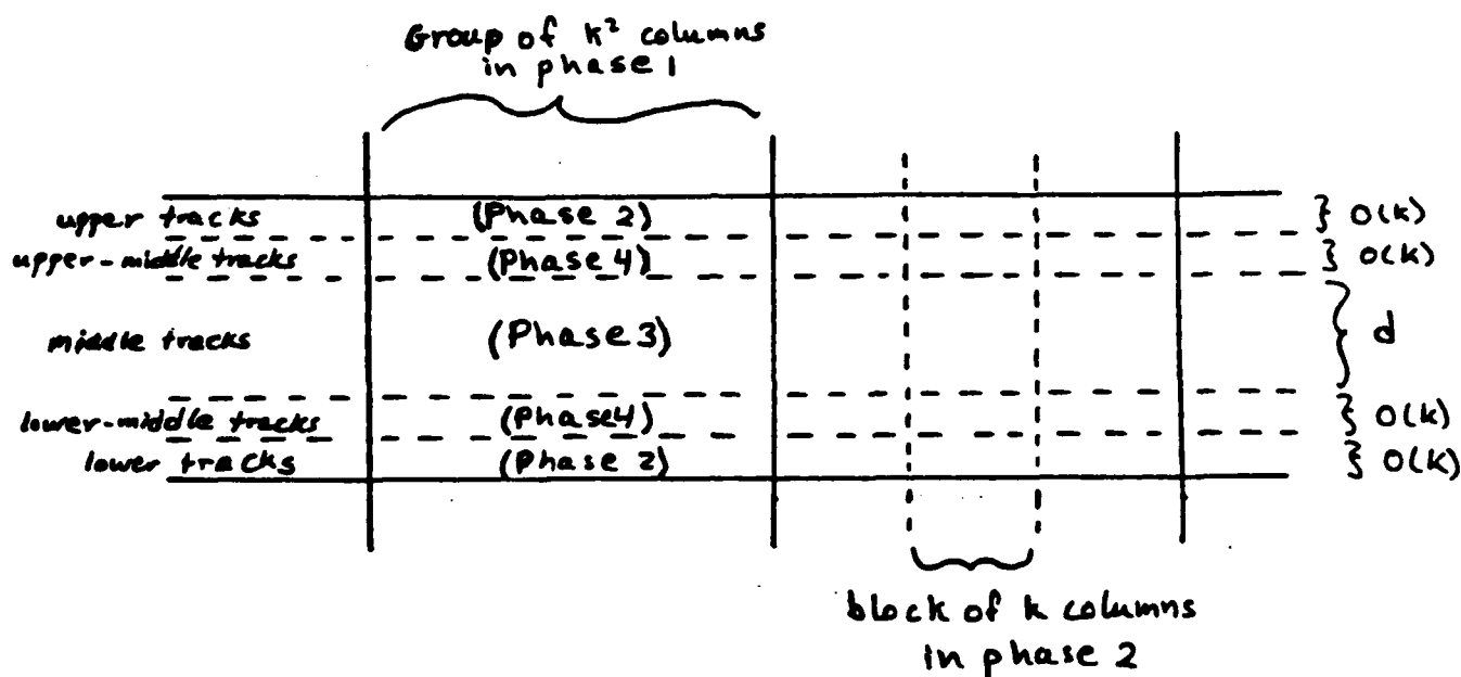
Figure 5: Illustration of the four phases of the algorithm.
