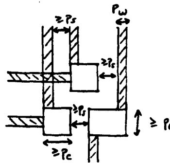
Figure 10: Design rules of the 3-parameter model.
