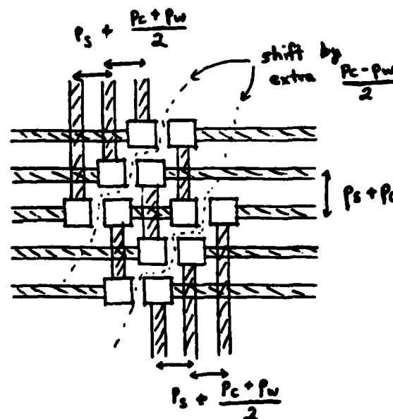
Figure 11: Spacing between successive staircases.
