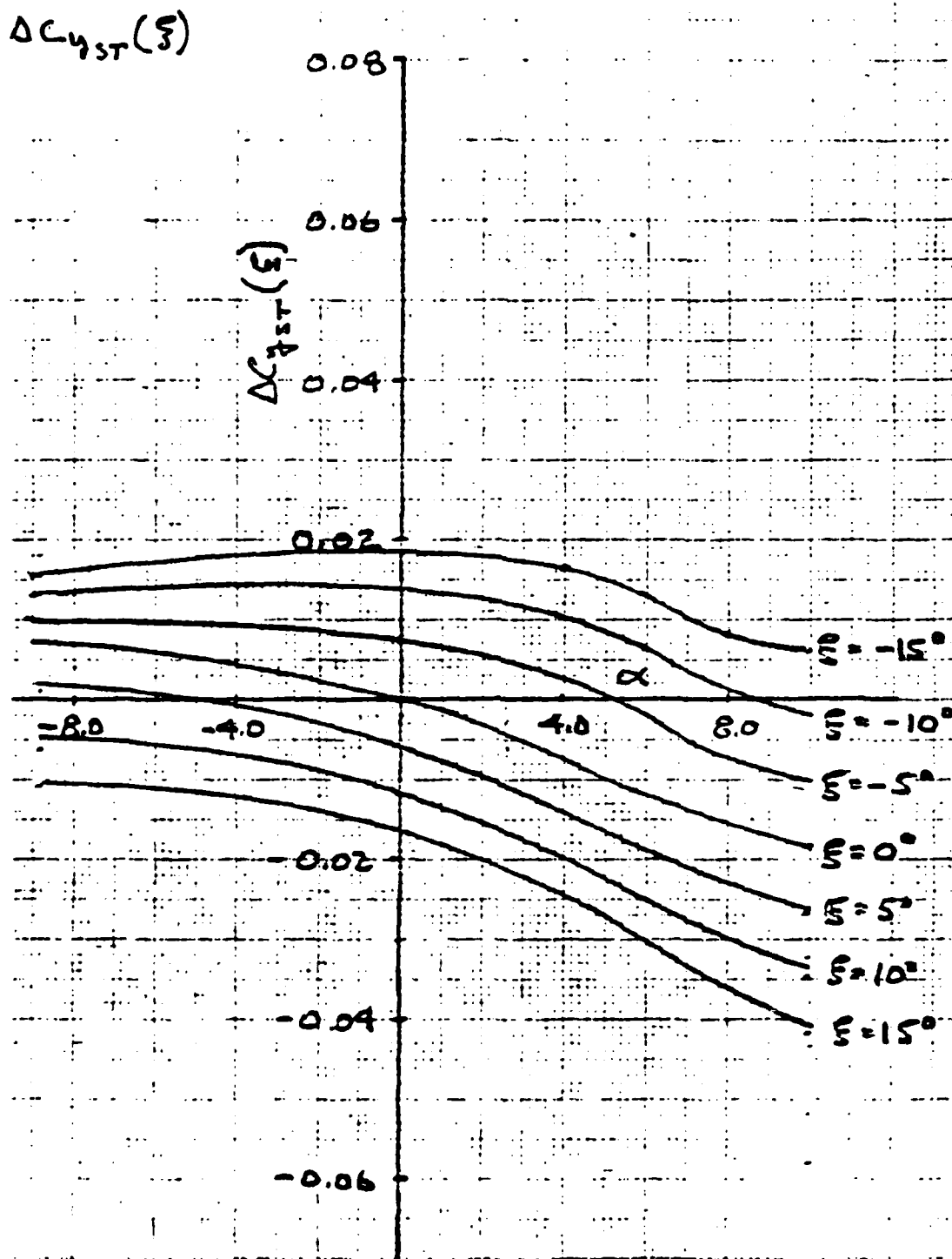
Lateral Control Characteristics \alpha vs \xi vs \Delta C_{YST}(\xi)
