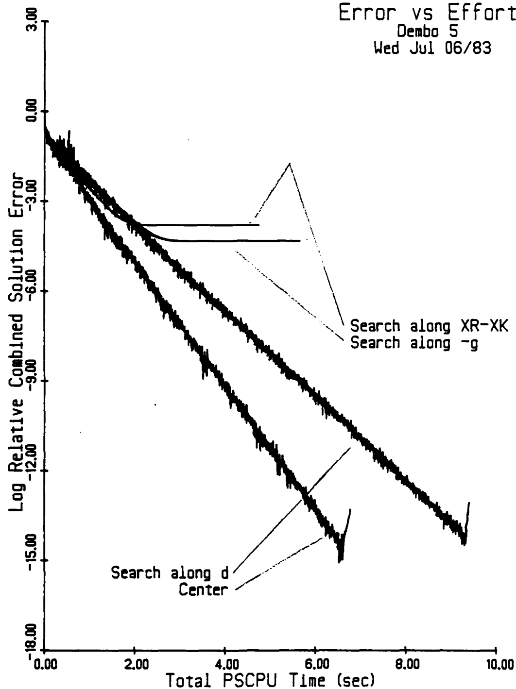
Figure D3.10 Dem 5: Deep Cuts Using Linesearches
