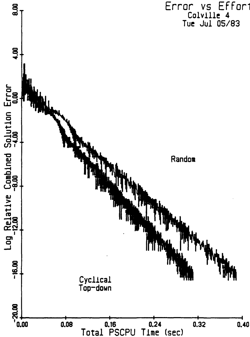
Figure D4.4 Col 4: Three Simple Strategies
