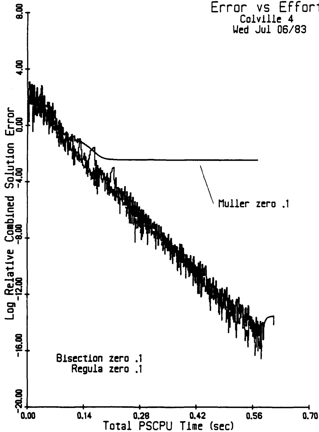
Figure D2.14 Col 4: Zero-finding at 0.1
