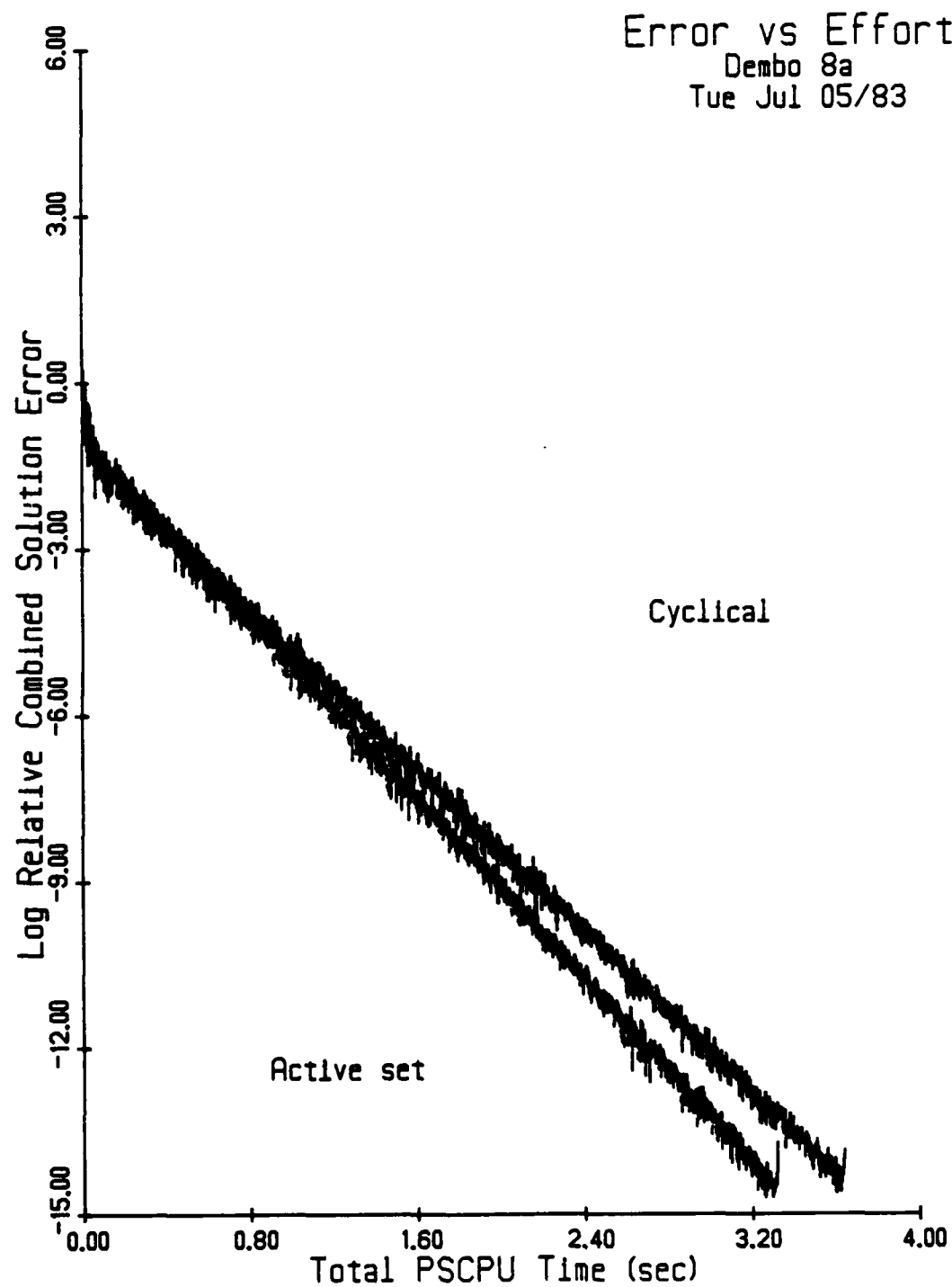
Figure D5.13 Dem 8: Active Set Strategy
