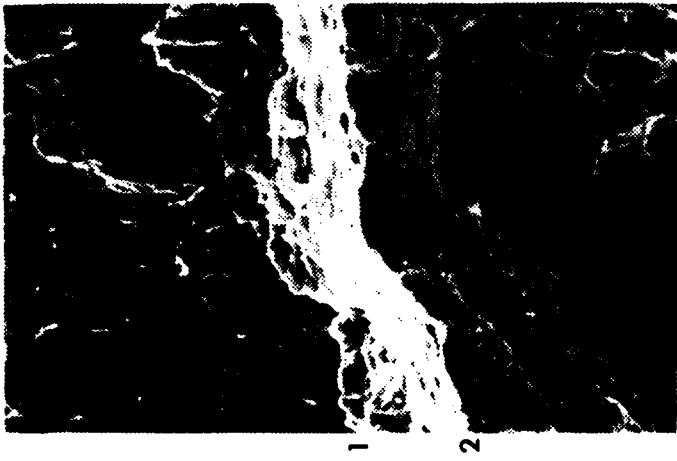
Sample Y 5% Prestrain, J_{Ic} = 737
