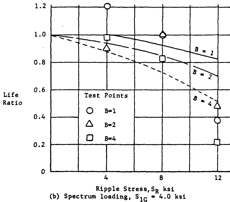
Figure 14 - Life Ratios; Comparison of Test Life vs. Sequence Accountable Analysis
