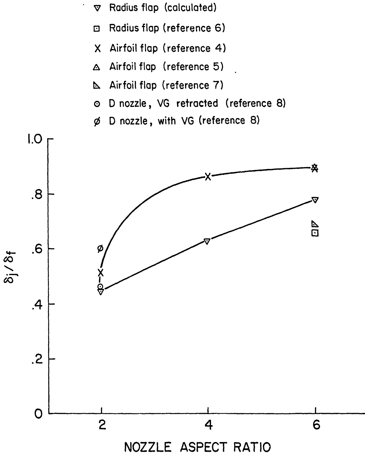
Figure 18 Static Turning Angle for Rectangular Nozzles and Various Flap Systems
