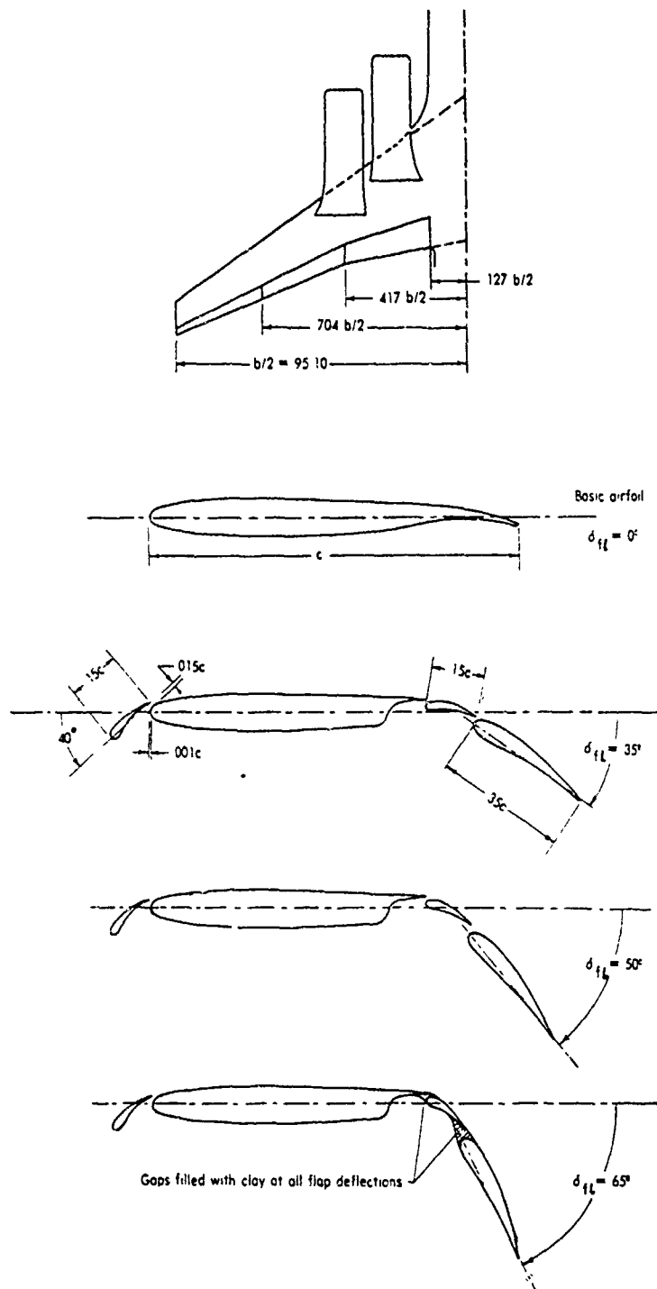
Figure 12 Basic High Lift System with Double-Slotted Flap
