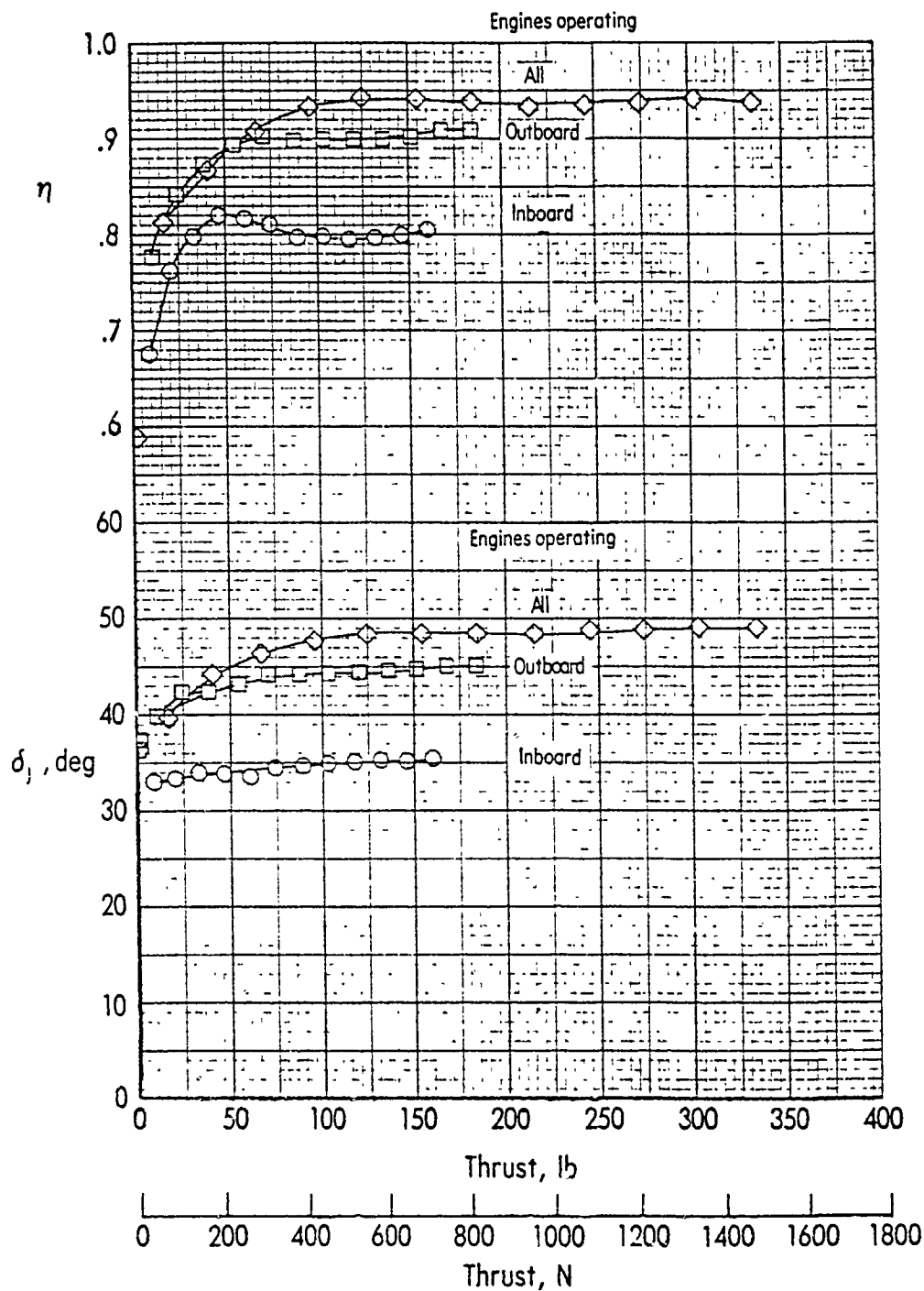
Figure 14 Variation of Static Turning Angle and Turning Efficiency with Twin-Engine Simulation. Rectangular Nozzles and Basic Flap
