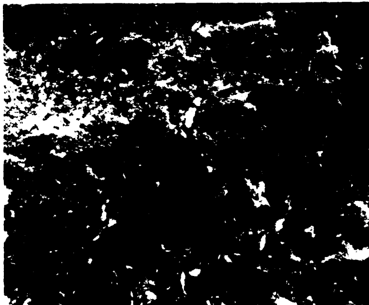
Figure 12. Micrograph 041383-4, X530. Microstructure of Plug 1 grout at 3 years. This sample came from a piece of a cylinder. Three grains of unhydrated cement can be seen in the right central portion of the micrograph. Note the microstructure appears denser than the same grout at 370-days age (Figure 6)
