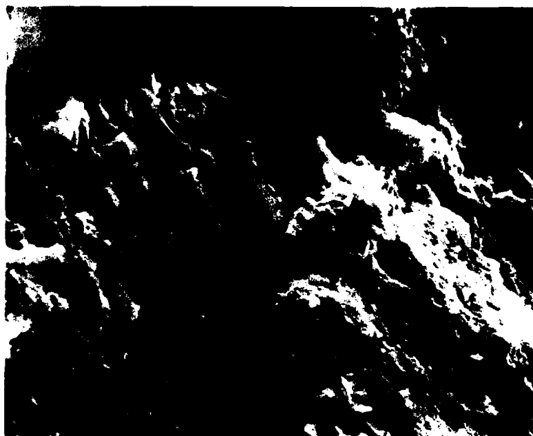
Figure 8. Micrograph 030581-26, X1900. Broken surface of Plug 2 cube CL-30 GRT-158. An unhydrated cement grain is seen in the upper left corner, bordered by calcium hydroxide and calcium silicate hydrate. The specimen was about 1 year old
