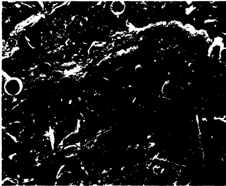
Figure 13. Micrograph 041383-15, X510. Microstructure of Plug 2 grout at 3 years. This sample came from cube CL-30 GRT-158 grout. The surface of this grout looks denser than Plug 1 grout of the same age (Figure 12). Unhydrated portland cement and fly ash spheres can be seen in the micrograph. A broken fly ash sphere is in the upper central portion of the micrograph
