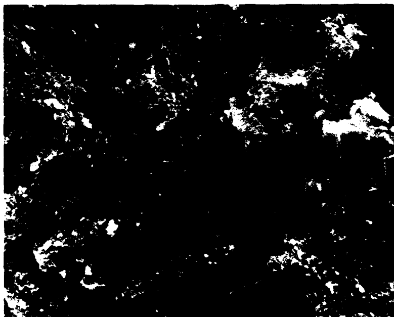
Figure 10. Micrograph 030581-10, X2000. Broken surface of Plug 1 cube A4. This surface shows more porosity than the Plug 2 cube surface (Figures 8, 9). The sample was about 18 months old
