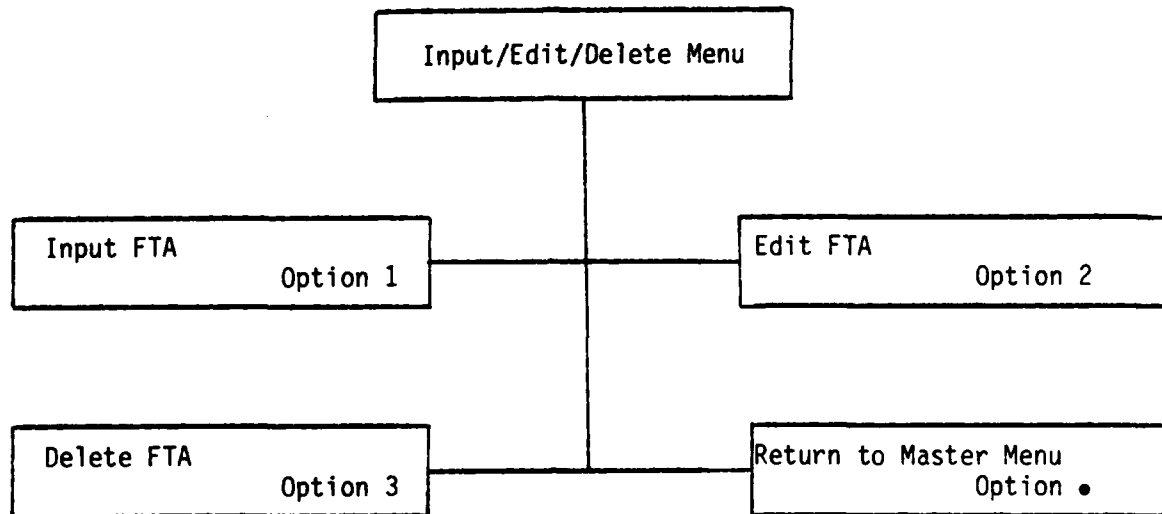
Figure 4. Input/Edit/Delete Subsystem
