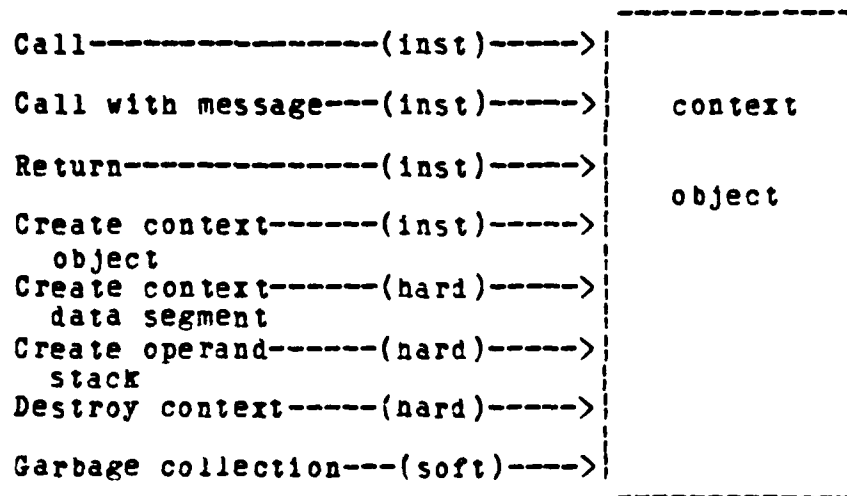
Figure 3.16 Context Object.
